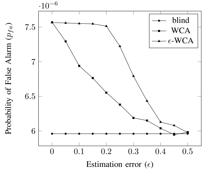
Figure 2. Estimation of the false alarm probability w.r.t the estimation error \epsilon for three attacks: WCA, \epsilon -WCA and blind. Parameters: m = 400 , T = 80 , c = 4 .
