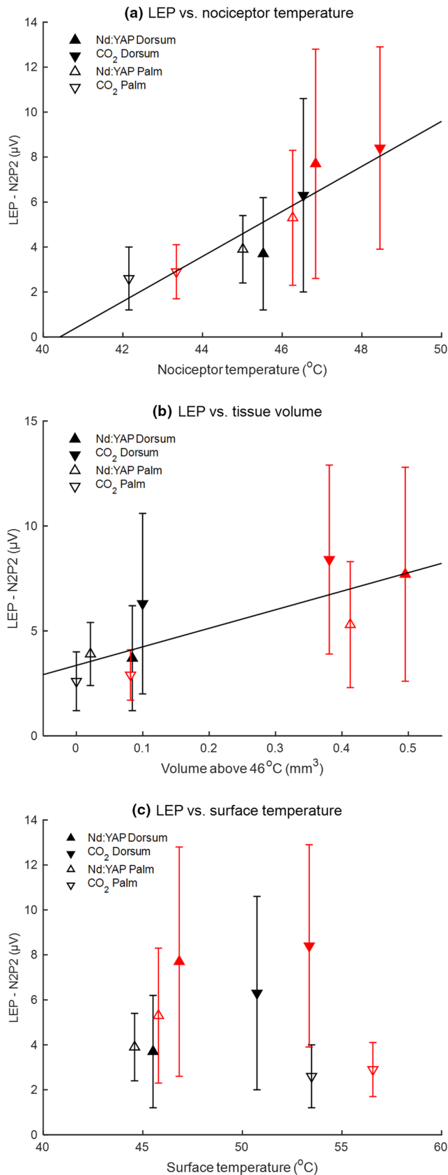
FIGURE 5 Correlation between LEP amplitudes (N2P2), indicated as mean \pm SD, and (a) the simulated maximum temperature at the DEJ of the simulated tissue, (b) the simulated tissue volume above A \delta threshold ( \geq 46^{\circ} C) and (c) the simulated maximum surface temperature. There was a significant correlation for both (a) and (b), but not (c). (a) The black line indicates the linear correlation between LEP amplitude and nociceptor temperature ( p < 0.01 , r = 0.92 ). (b) The black line indicates the correlation between LEP amplitude and tissue volume above threshold ( p < 0.05 , r = 0.80 ). (c) A linear regression analysis between LEP amplitude and skin surface temperature showed no significant relationship ( p = 0.80 , r = -0.11 ), indicating that skin surface temperature is not a good predictor of LEP amplitude. Colours refer to stimulation intensity (black: low intensity, red: high intensity).
