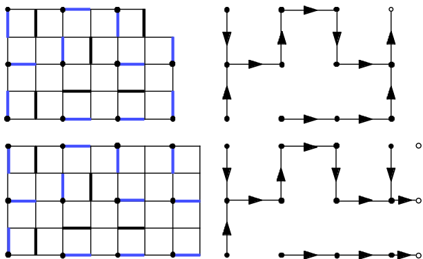
FIG. 1: (Color) Mapping of a dimer covering to a spanning tree on the odd sublattice, for an M \times N = 5 \times 7 lattice (top), and a 5 \times 8 lattice (bottom). In both cases, the solid dots represent the sites of the odd sublattice \mathcal{G} , and the open dots are the roots of the trees.
