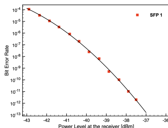
Figure 12. ORCA Bit Error Rate as function of power level of the receiver for the optical module data channel onshore. Black line is drawn just to guide the eye.
