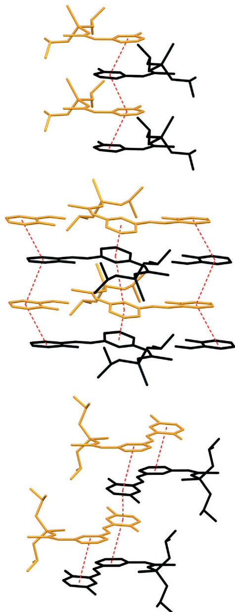
Fig. 6 Best stick views of the crystal packing of 1 (top), 2 (middle) and 3 (bottom). The crystal packing of 4–6 is similar to 3 . H-atoms were omitted for clarity.
