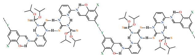
Chart 2 The simplified line diagram of dihalogen interactions in the structures of 3 (X = H, Y = Cl), 4 (X = H, Y = Br) and 5 (X = Y = Cl).
