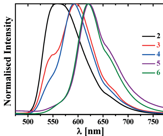
Fig. 8 Normalised solid-state emission spectra of 2–6 at 298 K ( \lambda_{\text{exc}} = 400 nm).
