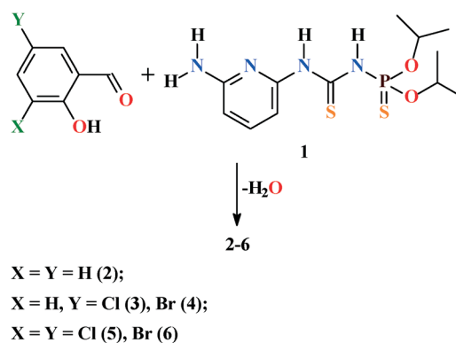
Scheme 1 Preparation of 2–6.
