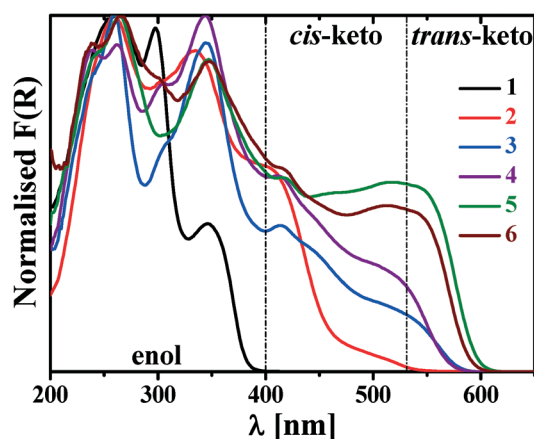
Fig. 7 Normalised Kubelka–Munk spectra of 1–6 at 298 K.
