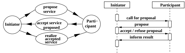
Figure 1. Call-For-Proposal Pattern
