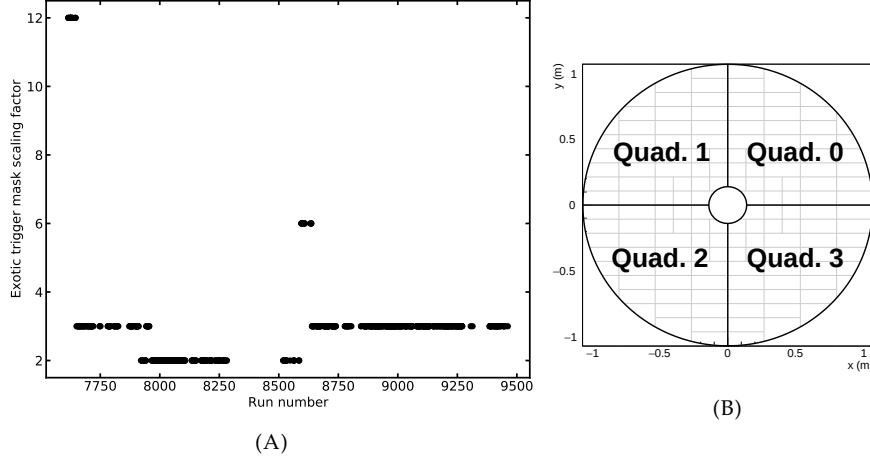
FIGURE 4.2: (A) Downscaling factor of the Dimuon trigger stream in the 2017 and 2018 data taking periods. Typically a value of 3 or 2 was used. The changes in the downscaling mostly overlap with modifications in the trigger definitions. (B) Map of the Charged Hodoscope (CHOD) quadrants which are used for the L0 trigger definitions.
