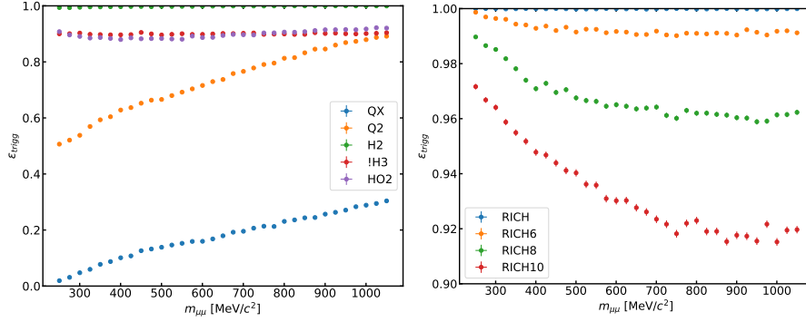
FIGURE 4.18: Efficiencies of the proposed L0 trigger conditions as a function of the ALP mass measured on the signal Monte Carlo. No pileup tracks were added, and no lifetime-related weight was applied. The H02 CHOD condition seems to be the best candidate to replace Q2 and QX. The trigger rate can be further adjusted using one of the RICH conditions shown on the right plot.
