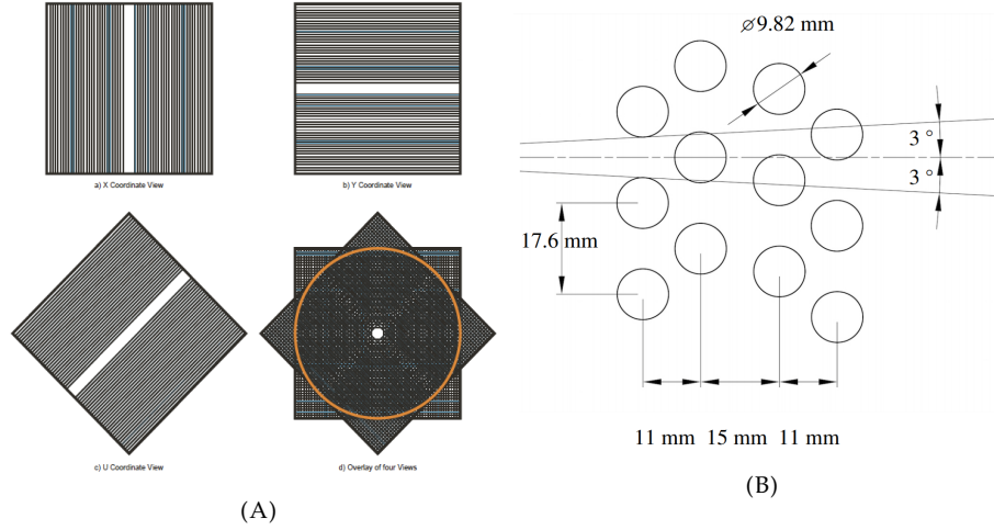
FIGURE 2.12: (A) One STRAW chamber composed of four views: X, Y, U, and V. In the middle of each view, a few straws are removed to create a passage for the beam pipe. (B) Straw geometry inside one view. It is based on two double layers with sufficient overlap to guarantee at least two straws to be crossed per view per track. Figures are taken from [108].
