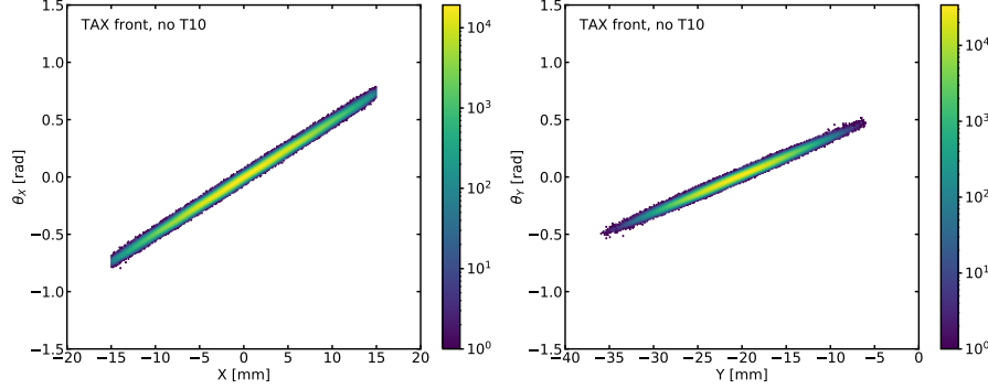
FIGURE 4.5: Angular distribution of protons as a function of the impact position at the TAX front plane. Angles and positions in the X-axis are shown in the left plot, while Y-axis is demonstrated on the right. The plots were obtained with the help of the dedicated beamline simulation described in [168].
