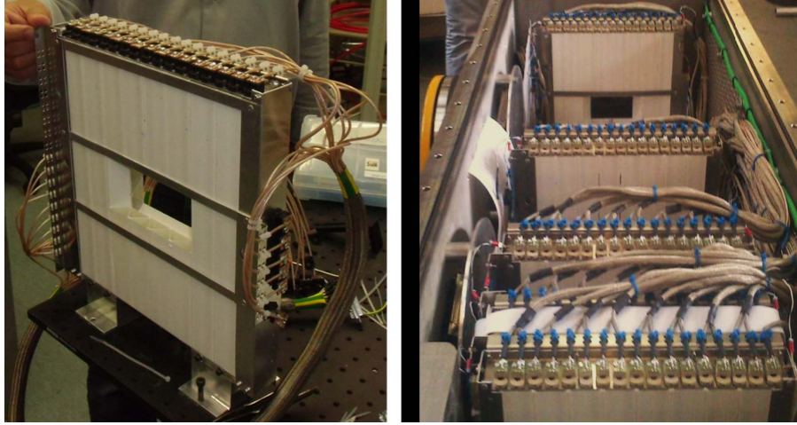
FIGURE 2.10: Left: Photo of a single CHANTI station. Right: View of the upstream part of the CHANTI vacuum vessel with the first five stations installed [108].
