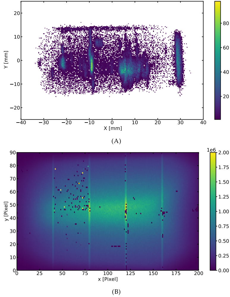
FIGURE 3.10: (A) Example of the map of missed hits at GTK1 extracted using data from run 8252, 2017 data sample. The inefficient areas should be compared with the hit map of the same station made for the same run and shown in Fig. (B). Note that the coordinate axes in Fig. (A) are rotated by 180^\circ with respect to those in Fig. (B). Comparing the two figures, one can see that the inefficiencies correspond to the dead or noisy pixels and areas outside the detector acceptance.
