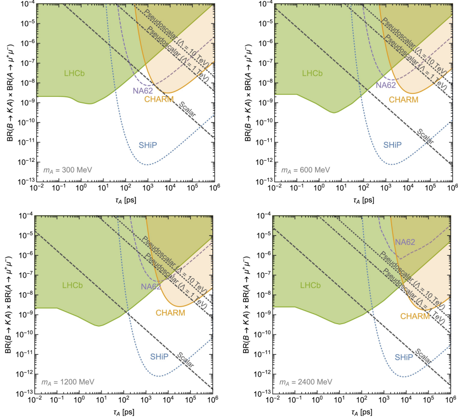
FIGURE 4.1: Model-independent constraints at 95% confidence level on the production and decay of a light pseudoscalar or a scalar expressed in terms of \mathcal{B}(B \rightarrow KA) \times \mathcal{B}(A \rightarrow \mu^+\mu^-) as a function of lifetime \tau_A for four masses: 300 MeV/ c^2 , 600 MeV/ c^2 , 1200 MeV/ c^2 and 2400 MeV/ c^2 [94]. Specific model-dependent predictions are shown as straight lines. NA62 appears to be the most sensitive for masses below 1000 MeV/ c^2 and lifetimes around 1000 ps.
