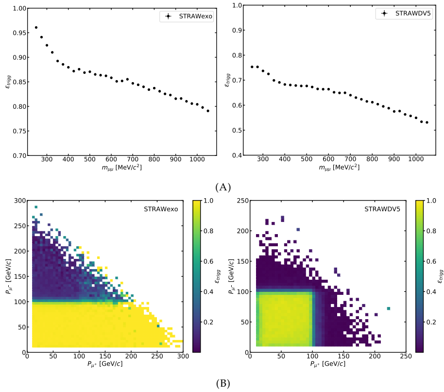
FIGURE 4.15: L1 trigger efficiencies measured on the signal Monte Carlo as a function of the mass of the generated particle (A) and the muon track momenta (B). No pileup tracks were added, and no lifetime-related weight was applied. Similarly to L0, the efficiencies were defined as a fraction of events passing the L1 algorithm and the signal selection from all events passing the signal selection.
