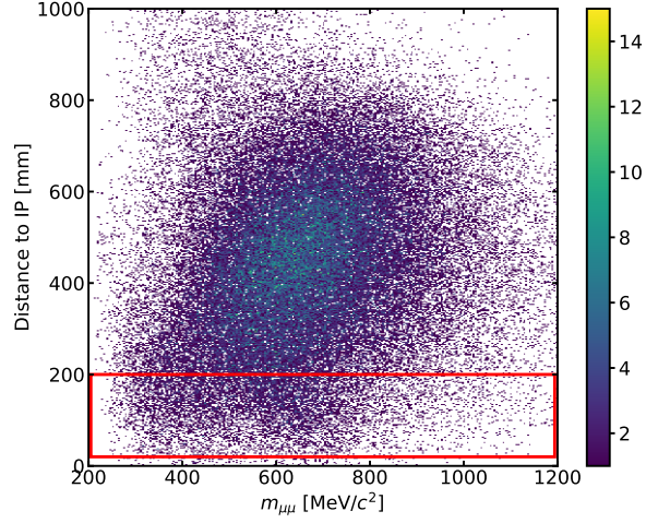
FIGURE 4.20: Minimum distance to the impact point (IP) as a function of the dimuon mass for events in the NA48 CHOD side-bands. The region used to extract the shape of the combinatorial background inside the signal region is shown with the red rectangle.
