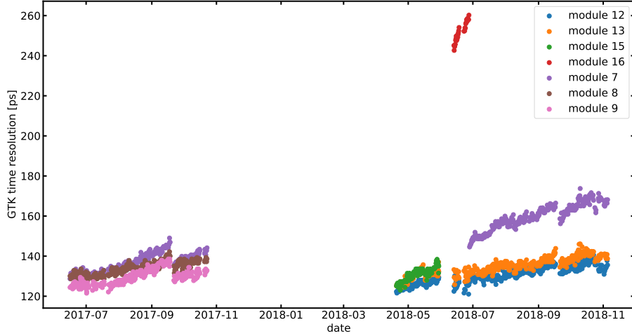
FIGURE 3.12: Single hit time resolution of each GTK module installed in 2017-2018. A moderate increase of about 20 ps can be seen by the end of each data taking period. All sensors except for the one used in module 16 are n-in-p.
