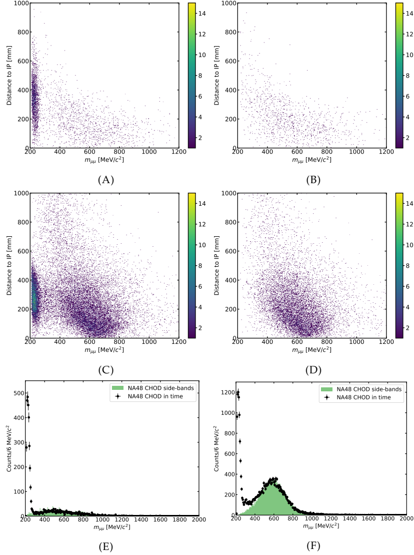
FIGURE 4.25: Top two rows: minimum distance to the impact point (IP) as a function of the dimuon mass for events inside the vertex Z position side-bands for \mu^+\mu^+ (top) and \mu^+\mu^- (middle) vertices: (A), (C) in time events; (B), (D) events in the NA48 CHOD side-bands. Bottom row: comparison between the dimuon mass distribution of the in time events and the events in the NA48 CHOD side-bands for \mu^+\mu^+ (E) and \mu^+\mu^- (F) vertices inside the vertex Z position side-bands.
