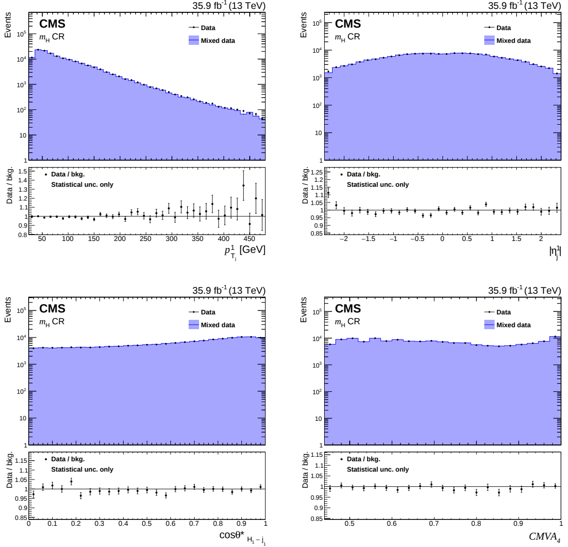
Figure 4: Comparison between the background model obtained with the hemisphere mixing technique and data in the m_H CR for the variables p_{T_1}^1 (upper left), \eta_1^1 (upper right), \cos\theta_{H_1-j_1}^* (lower left), and CMVA_4 (lower right). Bias correction for the background model, described in Section 8.2, is applied by rescaling the weight of each event using the event yield ratio between corrected and uncorrected BDT distributions in this CR. Only statistical uncertainties are shown as the uncertainties related to the bias correction can not be propagated from the BDT classifier to a different variable.
