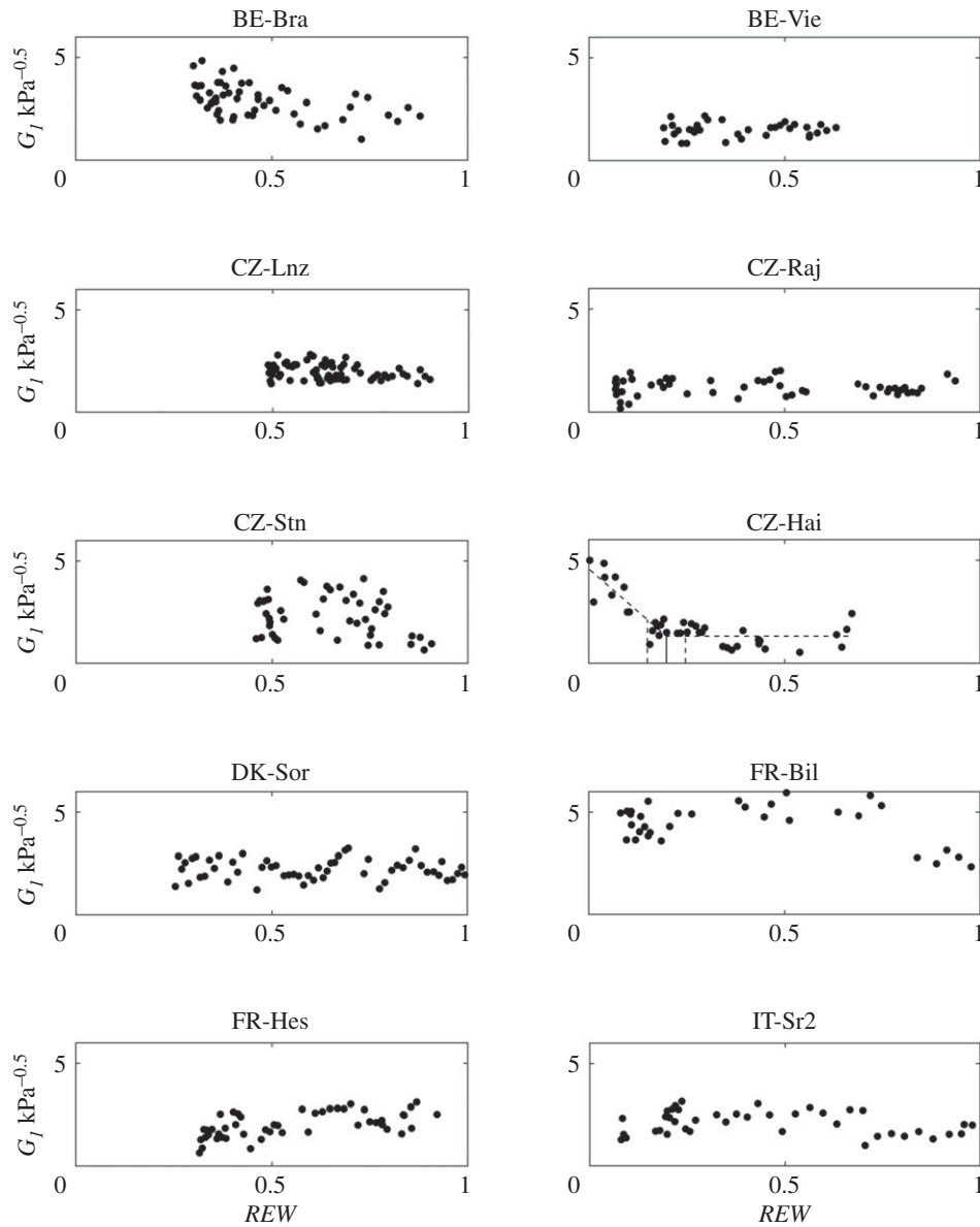
Figure 2. Dependence of G_1 on REW for each site. REW_{b,G1} are marked by a vertical solid line with 95% confidence intervals (dashed vertical lines). Regression lines are only shown when F -test p -values (comparison with linear regression) were smaller than 0.05.
