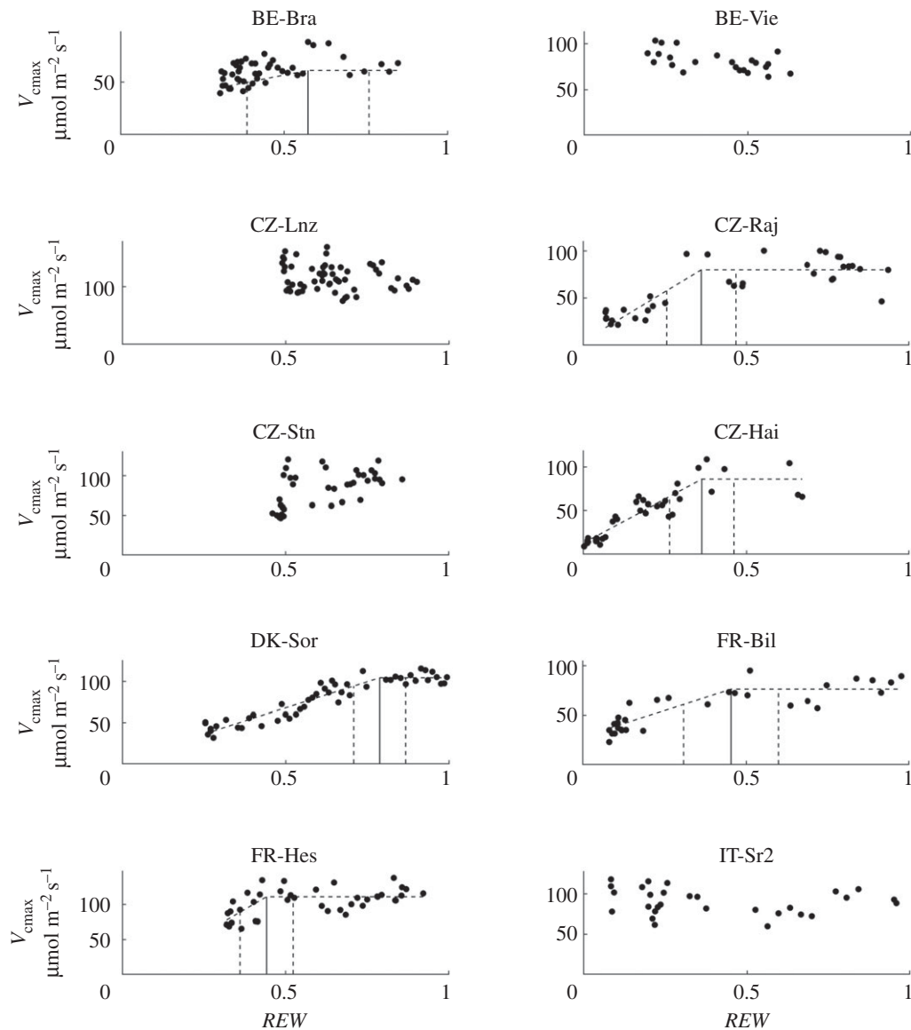
Figure 3. Dependence of V_{\text{CMAX,APP}} normalized at 25°C on \text{REW} for each site. \text{REW}_{B,VC\text{MAX}} are marked by a vertical solid line with 95% confidence intervals (dashed vertical lines). Regression lines are only shown when F -test p -values (comparison with linear regression) were smaller than 0.05.
