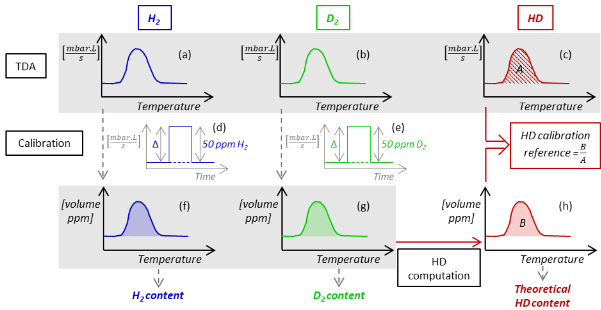
Figure 3 – Schematic representation of the methodology developed to compare experimental results and theoretical computations.
