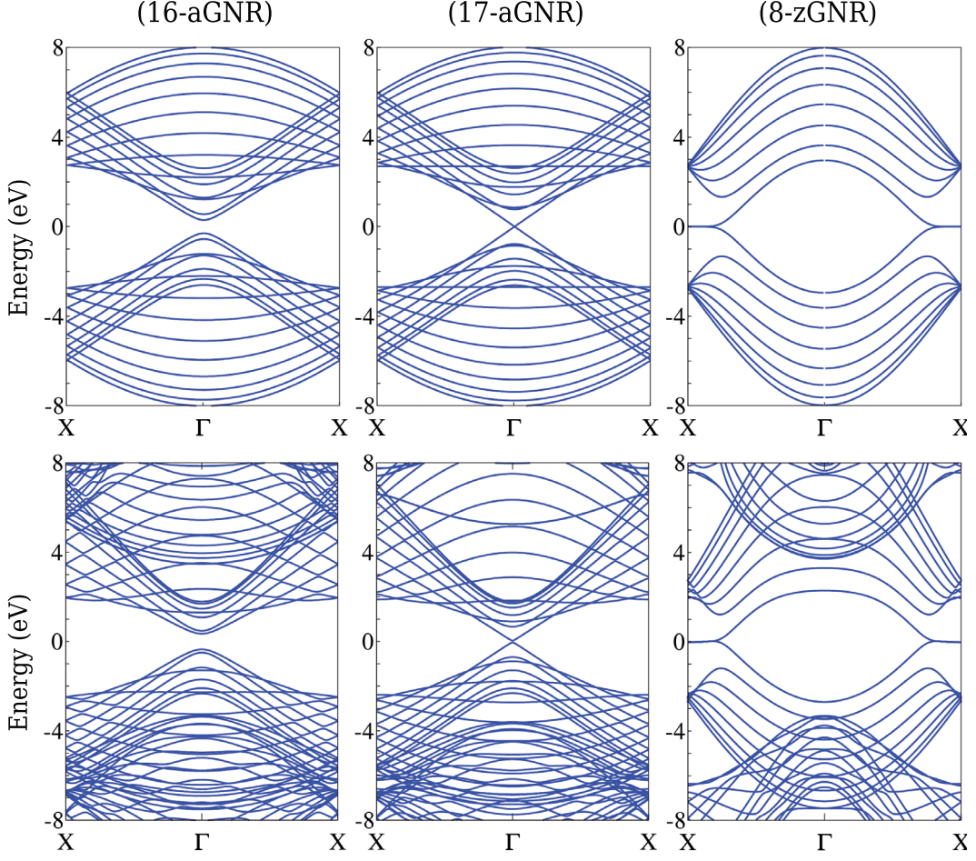
Fig. 9. Energy band structures of two armchair nanoribbons ( N -aGNRs) of various width ( N = 16, 17 ) and one zigzag nanoribbon (8-zGNR). The tight-binding band structures (top) computed using a constant hopping energy ( \gamma_0 = 2.7 eV) between nearest neighbors are compared to ab initio band structures (bottom).
