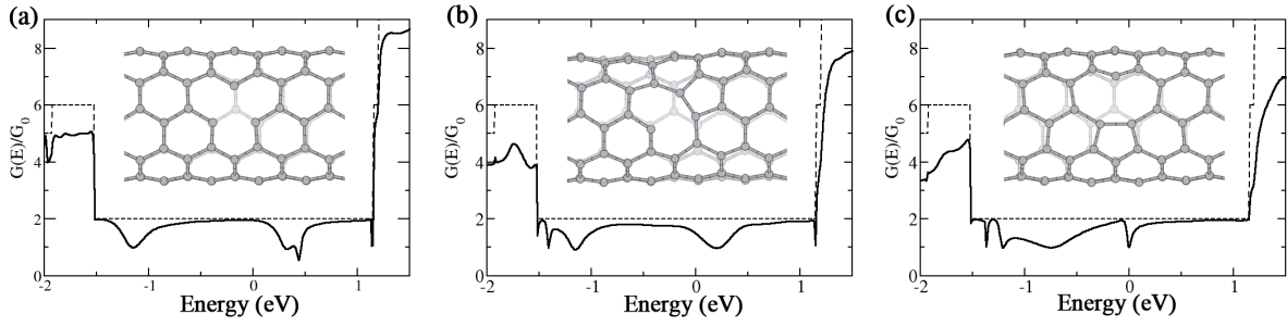
Fig. 19. Quantum ab initio conductance of a (5,5) armchair nanotube containing (a) a bare D_{3h} monovacancy and a reconstructed C_s vacancy in two different positions: (b) tilted or (c) perpendicular to the axis of the tube. Atomic structures of the corresponding defects are shown in insets.
