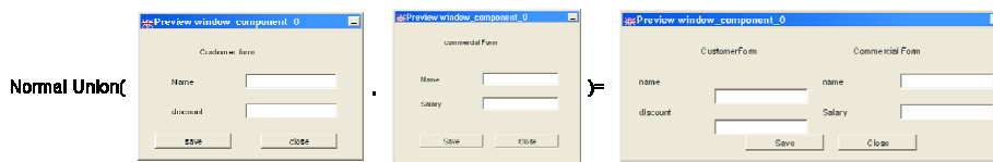
Fig. 6. An example of expected user interfaces from union of the two user interfaces
