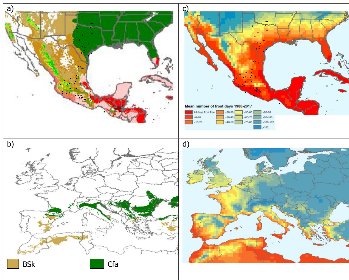
Figure B.1: Koppen–Geiger climate types and mean number of frost days in North and Central America which were visually compared to Europe (see Section 3.4.3 for detail). Black dots in (a) and (c) indicate occurrence of D. virgifera zea (from Krysan et al., 1980)
