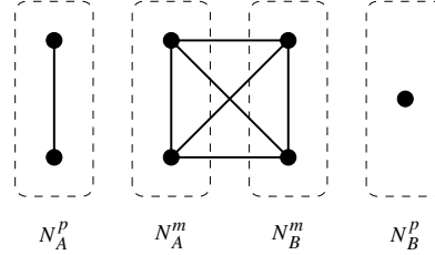
Fig. 6. RCPS network in Corollary 2 in which \hat{N}_A^P = \hat{N}_B^P = \emptyset , for n = 7 . Public links are indicated by solid lines and shadow links by dashed lines.
