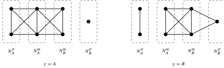
Fig. 5. PS networks in Proposition 3 (iii) for n = 7 .
