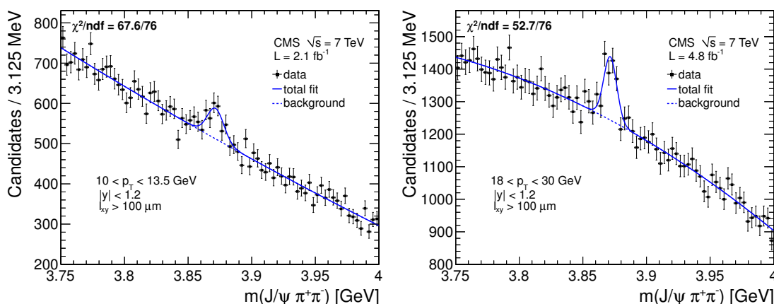
Figure 4. The J/\psi\pi^+\pi^- invariant-mass distribution in the X(3872) region for p_T = 10 –13.5 GeV (left) and 18–30 GeV (right) in a B-enriched sample. The lines represent the signal-plus-background fits (solid) and the background-only components (dashed). The \chi^2/\text{ndf} of the fit is also reported.
