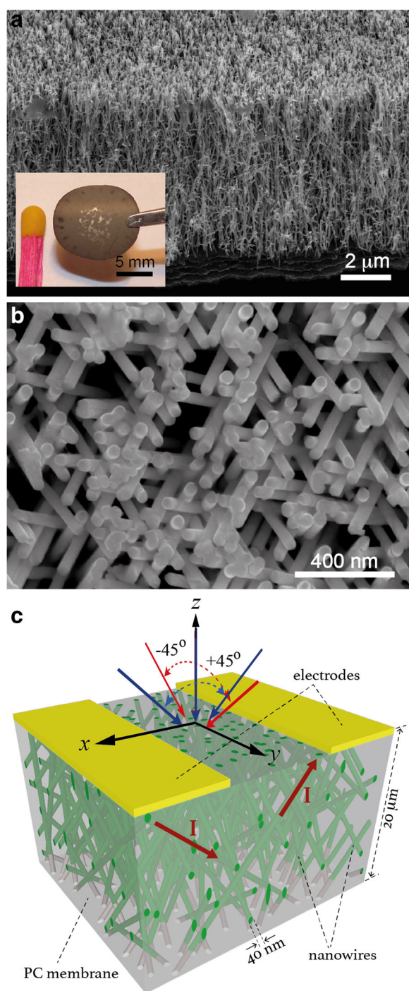
Fig. 1 a Low-magnification tilted view SEM image of an interconnected network of electrodeposited 3D Ni CNWs, with NW diameter of 40 nm, obtained after complete dissolution of the host PC membrane. The inset displays an optical image showing the size and mechanical robustness of the macroscopic self-supporting network. b Top view of the dense Ni CNW network of a . c Schematic representation of a 3D PC membrane featuring cylindrical nanopores with a mean diameter of 40 nm and partially filled with CNWs. An electrode design for two-probe electrical measurement is also shown
