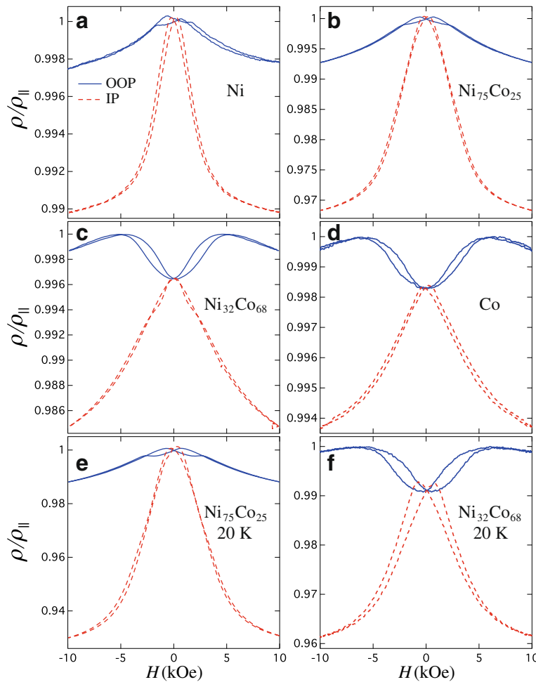
Fig. 4 Magnetoresistance curves for \text{Ni}_x\text{Co}_{1-x} ( 0 \leq x \leq 1 ) CNW networks measured a–d at 290 K and e, f at 20 K, by applying the external field in the OOP (continuous lines) and IP (dashed lines) directions
