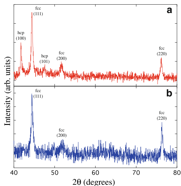
Fig. 3 X-ray diffraction patterns of a the Ni 32 Co 68 and b Ni 75 Co 25
