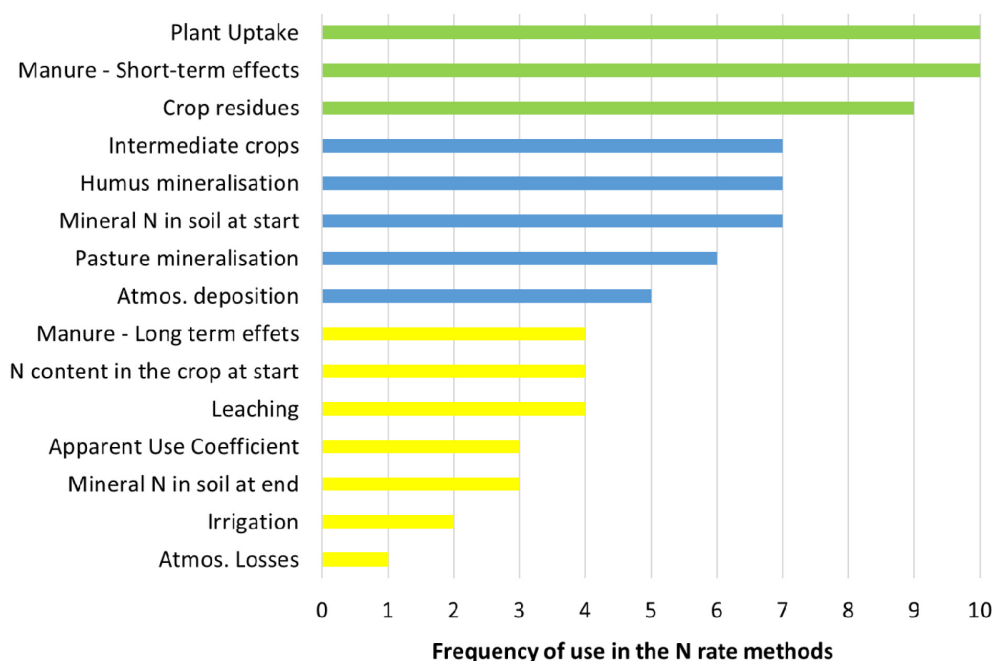
FIGURE 1 Decreasing frequency of the variables used in the methods of calculation of the recommended nitrogen fertilisation rates. Green: most shared variables. Yellow: least shared variables. Blue: intermediate.
