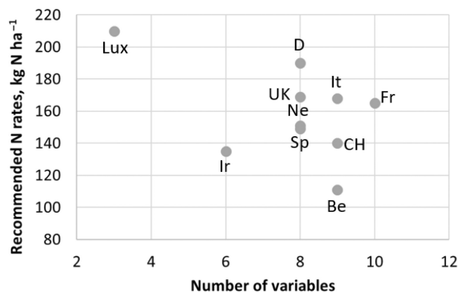
FIGURE 5 Relationship between the recommended N fertilisation rates (arable scenario) and the number of variables explicitly present in the fertilisation calculation methods. Belgium (Be), Germany (D), France (Fr), Ireland (Ir), Italy (It), Luxembourg (Lux), the Netherlands (Ne), Spain (Sp), Switzerland (CH) and United Kingdom (UK).
