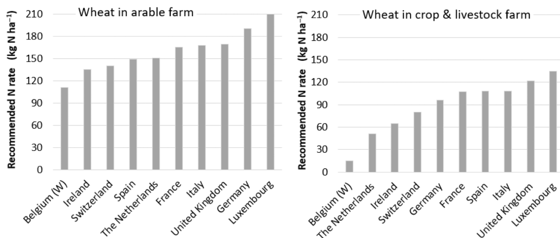
FIGURE 4 Recommended Nitrogen (N) fertilisation rates for 10 west European countries, calculated from the official national methods, and applied on a theoretical study case consisting of a wheat crop grown in two types of farming systems.
