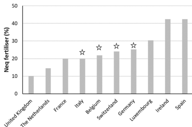
FIGURE 2 Percentage of N (from the farmyard manure use in the case study) considered to be available for the crop in the season after its spreading. Stars indicate the countries that take into account with a separate budget component a long-term effect (>1 year) of previous spreading on the soil N supply.
