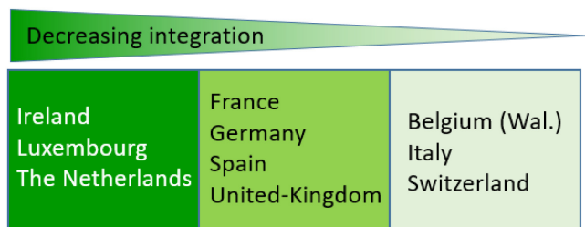
FIGURE 3 Countries ranked by decreasing integration of the fertiliser recommendations in their legal enforcement (from dark to clear green).
