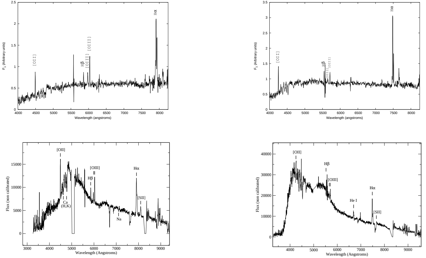
Fig. 14. 2dF spectra of two absorbed X-ray sources which only present narrow emission lines in their optical spectra (upper panel). These are sources #84 and #66 in Table 4, respectively. They have been classified as star forming galaxies, based on the line ratios inferred from their optical spectra. The lower panel show the optical spectra of the corresponding objects, obtained with the SALT. Both have been observed with the PG0300 grism ( R \sim 400 ). The SALT optical spectra are not flux calibrated.
