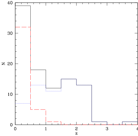
Fig. 1. Spectroscopic redshift distribution of the 99 optical counterparts in our sample. The solid histogram refers to the whole sample, the long-dashed histogram refers to type 2 AGN and the dotted histogram refers to type 1 AGN.
