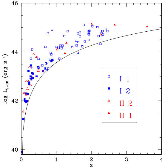
Fig. 10. 2-10 keV intrinsic rest-frame luminosities as a function of redshift for our sample of X-ray sources. Squares are X-ray sources classified as type I while triangles are those classified as type II. Filled symbols are the sources for which the X-ray and the optical classifications do not match. The solid line is showing the 2-10 keV luminosity as a function of redshift for a 2-10 keV limiting flux of 8 \times 10^{-15} \text{ erg s}^{-1} \text{ cm}^{-2} .
