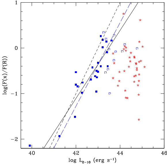
Fig. 12. X-ray to optical ratio (2-10 keV band vs R band) as a function of the deabsorbed, intrinsic 2-10 keV luminosity for the type I objects. Some of them are only presenting narrow emission lines (filled squares). The type I that show broad and obvious emission lines in their optical spectra are divided into two categories : those which lie at z < 0.8 (empty squares) and those at z > 0.8 (stars). The solid line represents the minimum \chi^2 fit between \log(F_X/F_{\text{opt}}) and \log L_{2-10} for our data. The short dashed line represents the best linear regression for type 2 AGN, obtained using the data of Fiore et al. (2003), and the long dashed line is from the data of Treister et al. (2005).
