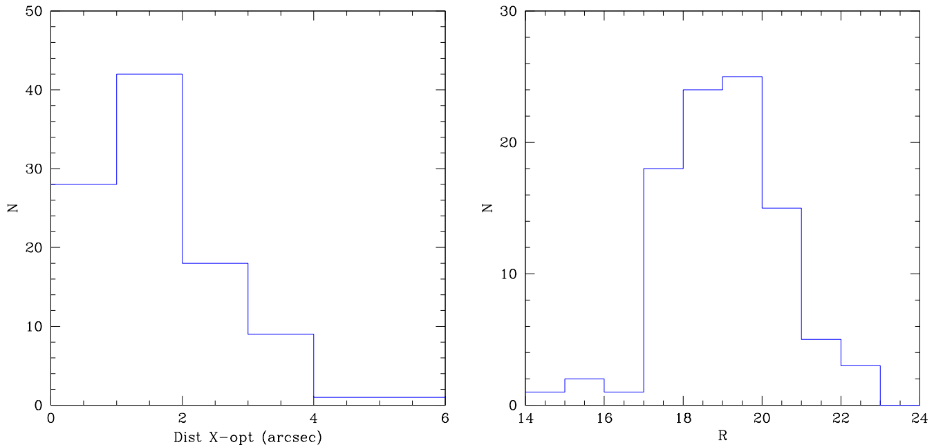
Fig. A.3. Left panel : histogram of the distribution of the separation between each X-ray source and its optical counterpart, for the 99 spectroscopically identified X-ray sources. Right panel : R band magnitude distribution of the 94 optical counterparts of our sample of X-ray sources for which an R band magnitude is available. For most of the objects, the magnitude is red magnitude from UKST plate scans, while the others are R magnitudes from the VVDS.
