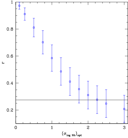
Fig. 5. The average value of the r coefficient over 100,000 simulations as a function of the standard deviation \sigma of the assumed gaussian distribution of the logarithm of the column density in the optical. The error bars for the r value correspond to 1\sigma . The solid line corresponds to the value r = 0.275 that we obtain for our sample of 99 X-ray sources.
