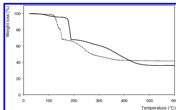
Figure 6. Thermogravimetric analyses of 1 (dashed line) and 2a (straight line) in air (10 °C/min).
