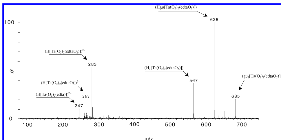
Figure 2. Negative ion mass spectrum of compound 2a in \text{CH}_3\text{OH}/\text{H}_2\text{O} .
