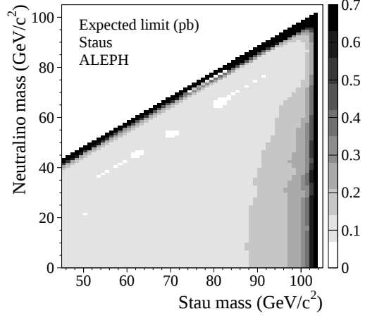
Figure 3: Upper limit at 95% C.L. on the observed (left) and expected (right) production cross section at \sqrt{s} = 208 GeV, times the branching ratio into \ell\chi_1^0 for (a) selectrons, (b) smuons and (c) staus.
