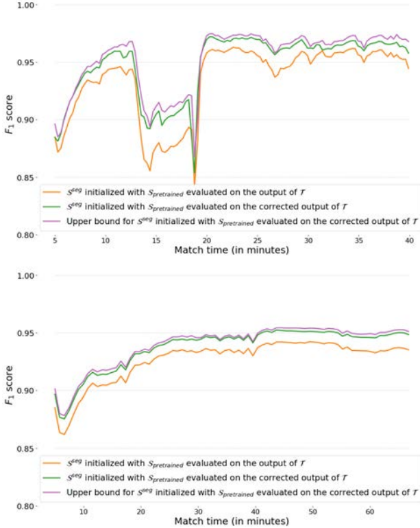
Figure 6. The previous curves (orange) are adjusted (green) by evaluating the instances S_k^{\text{seg}} ( k = 0, 1, \dots ) of S^{\text{seg}} on the manually corrected test frames for the soccer (top) and basketball (bottom) matches. The green curves are higher, which suggests that S^{\text{seg}} is right when T is wrong. The maximum performances that S^{\text{seg}} would achieve if we suppose that S^{\text{seg}} is correct when T is wrong are plotted in purple. Since the green and the purple curves are close, S^{\text{seg}} is almost perfect on the pixels mislabeled by T .
