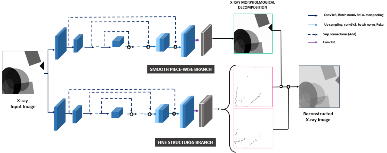
Figure 2: Overview of the network architecture. The network is composed of two main branches, one for the prediction of the piecewise component and the other for fine structures, both of which are based on a 6-layer deep U-Net with skip connections. The piecewise branch has one output channel whereas the fine structures branch has two output channels.
