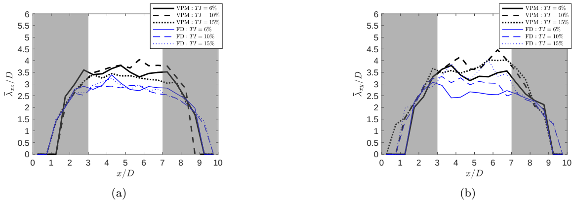
Figure 6. Mean binned wake centerlines wavelengths obtained by the VPM method (thick black line) and the FD code (thin blue line), in a horizontal ( z-x ) and in a vertical ( y-x ) plane, normalized by the rotor diameter ((a)-(b)) for several inflow turbulence intensities : TI = 6\% , TI = 10\% , and TI = 15\% ; note that the exploitable part of the graphs ranges between 3 \lesssim x/D \lesssim 7 because of the method used to determine the amplitude and wavelength of the oscillations
