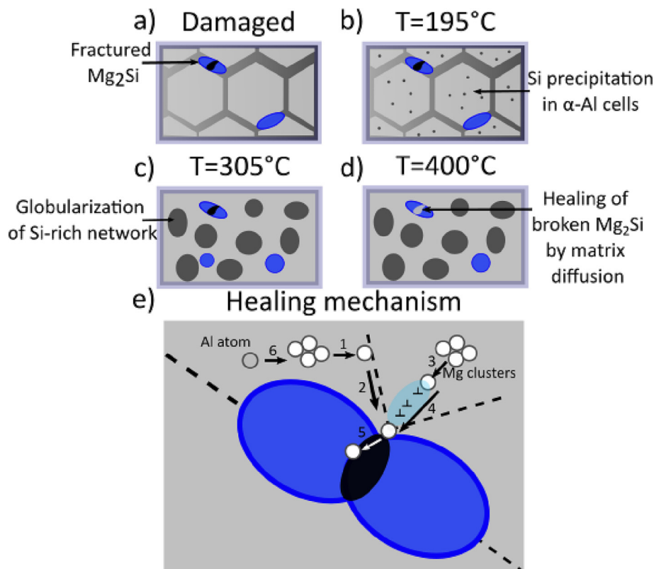
Fig. 7. Microstructure of \text{AlSi10.5Mg4} composed of \alpha\text{-Al} cells (light grey) surrounded by a Si-rich network (dark grey) and \text{Mg}_2\text{Si} particles (blue) a) in the damaged state and during the HHT when the temperature reaches b) 195 °C, c) 305 °C and d) 400 °C. e) Healing mechanism proposed for the \text{AlSi10.5Mg4} alloy: 1 – diffusion of Mg atoms from clusters to grain boundaries; 2 – grain boundary diffusion of Mg atoms to the crack tip; 3 – lattice diffusion of Mg atoms to a stress field area; 4 – dislocation pipe diffusion of Mg atoms to the crack tip; 5 – diffusion of Mg atoms to a flat plane of the crack; 6 – diffusion of Al atoms through the same path as Mg atoms.
