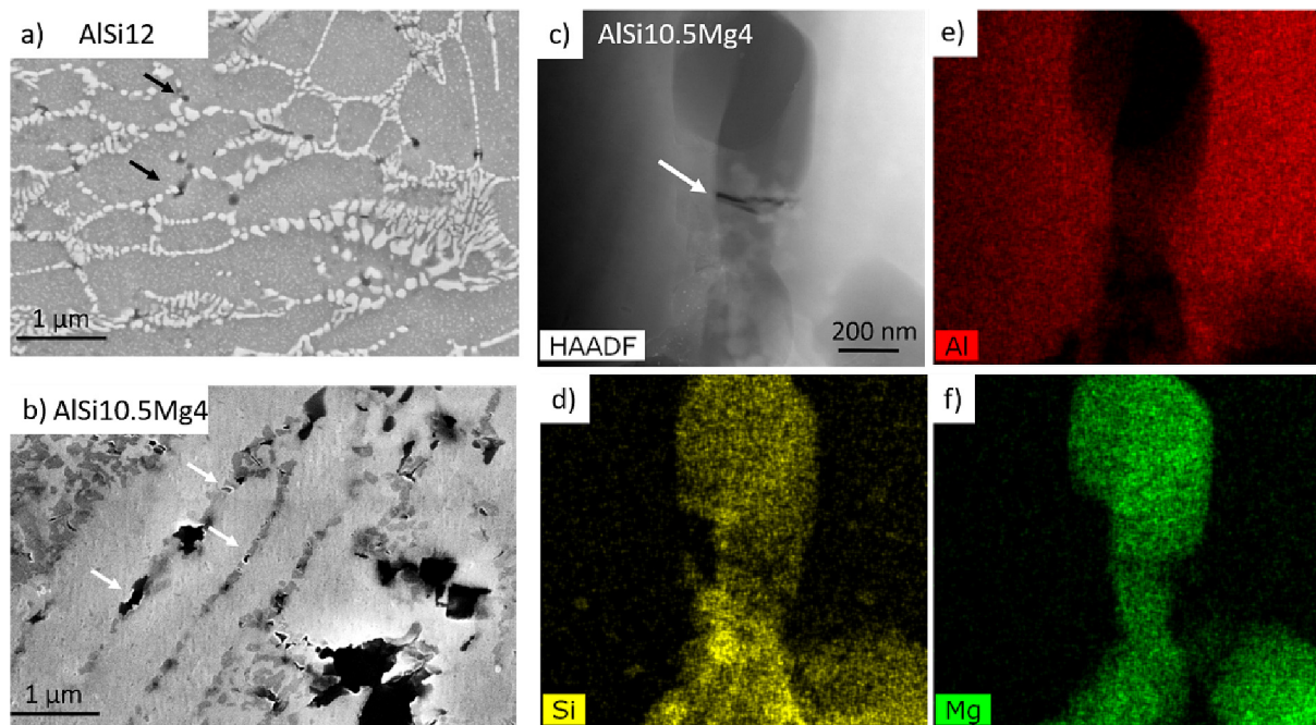
Fig. 3. SEM image of the mid-section of a fractured specimen of a) AlSi12 and b) AlSi10.5Mg4. c) TEM image of a fractured Mg_2Si particles in AlSi10.5Mg4 and its EDS elemental mapping of d) Si (in yellow), e) Al (in red) and f) Mg (in green). Arrows are drawn to highlight some damage sites. Note that the contrast between \alpha -Al cells and Si-rich network is inverted for AlSi12 and AlSi10.5Mg4 because AlSi12 was etched using Keller's reagent while this was not possible for AlSi10.5Mg4 due to Mg preferential etching.
