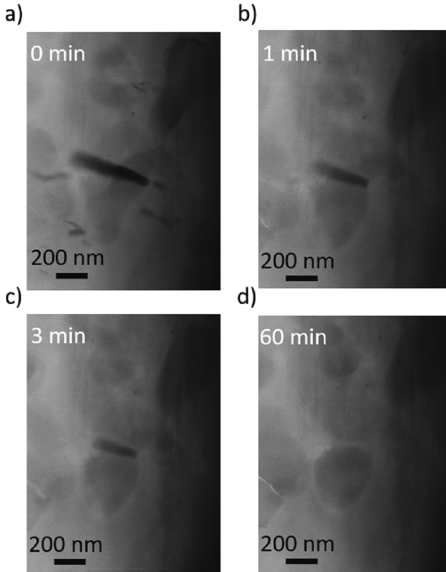
Fig. 5. STEM image of the evolution of a fractured \text{Mg}_2\text{Si} particle during a HHT at 400 °C after a) 0 min, b) 1 min, c) 3 min and d) 60 min.
