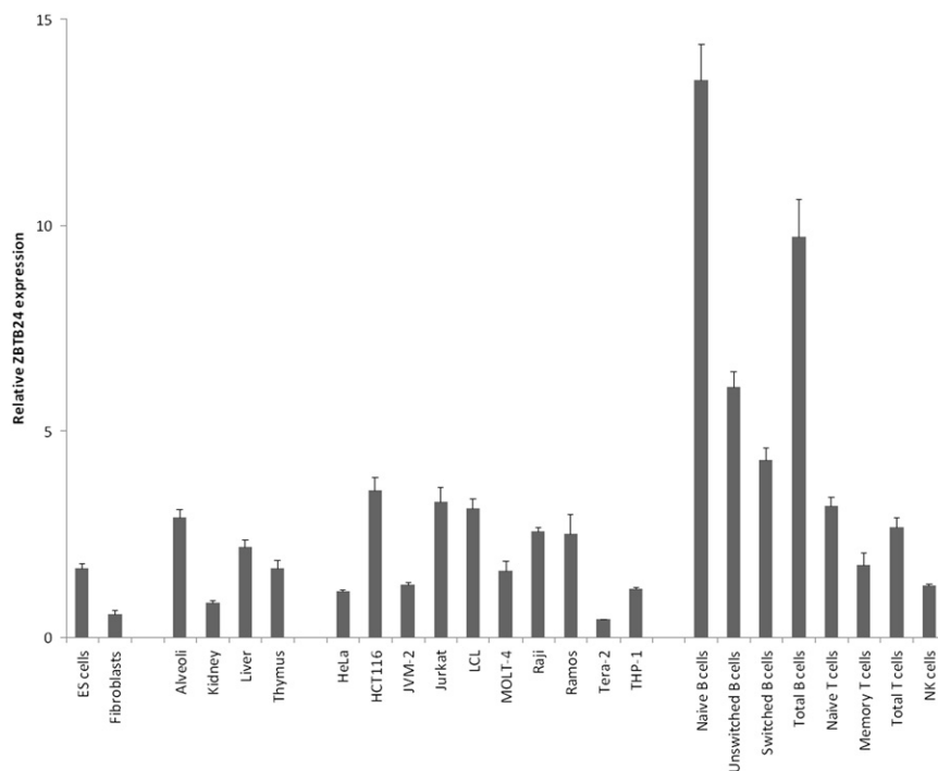
Figure 3. ZBTB24 Expression
