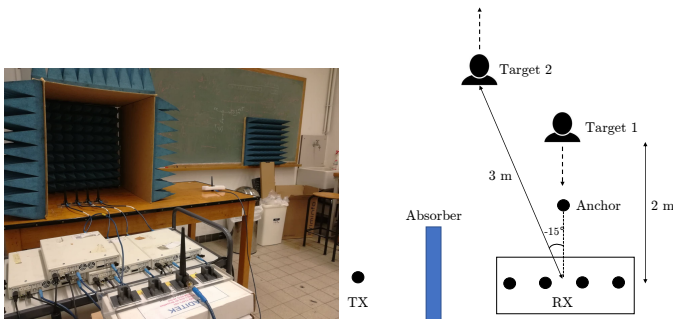
Fig. 1. Experimental setup
