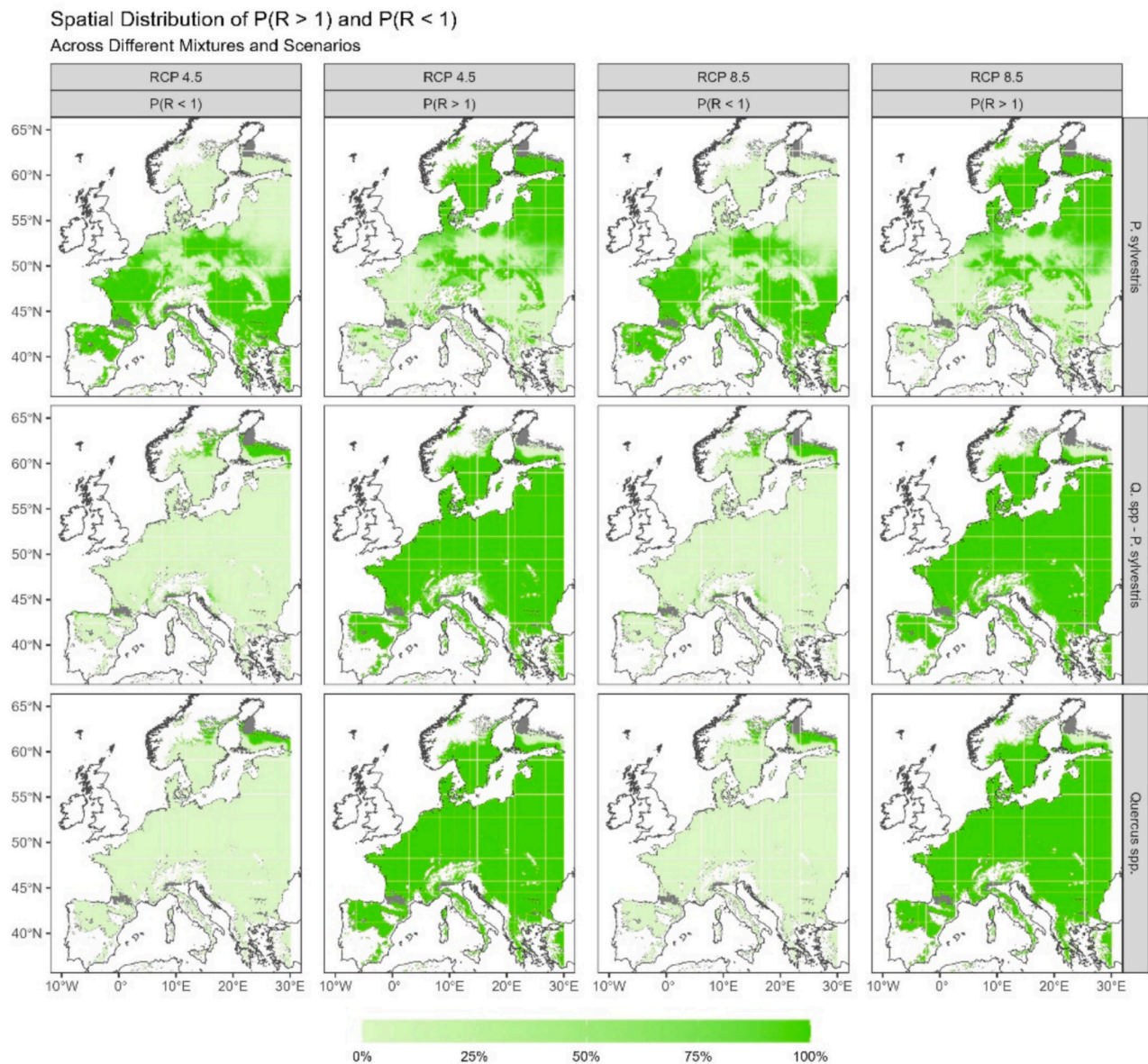
Fig. 6. Probability (0–100 %) of climatic response sum of future scenario (columns) exceeding, or becoming less suitable, than the historical scenario, by species-mixture (rows). Marked in grey are areas with only scenarios from a single GCM within a suitable distance from the climatologies which the triplet sites were exposed to during simulation. For full resolution, the reader is referred to the electronic print of this article.
