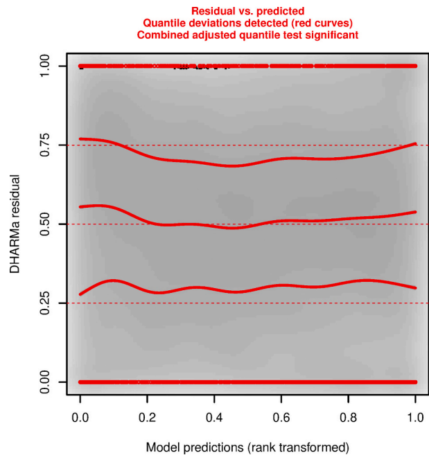
Fig. A3-1. Simulated residuals from the estimated Gamma distribution.
