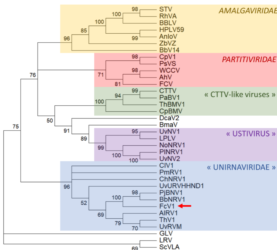
Figure 6. Phylogenetic placement of FcV1 ORF2 and related RdRp. The numbers next to nodes refer the percentage of bootstrap replicates that accommodates the branches together. Branches with bootstrap values <50% were collapsed. The position of FcV1 is highlighted by a red arrow. Members of the family Totiviridae : Giardia lamblia virus (GLV), Leishmania RNA virus (LRV) and Saccharomyces cerevisiae virus L-A (ScVLA) were taken to root the initial tree.
