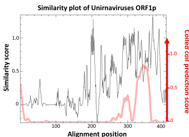
Figure 3. Similarity plot of aligned sequences of unirenaviruses ORF1p (black line) and CC prediction using Deepcoil (red line).
