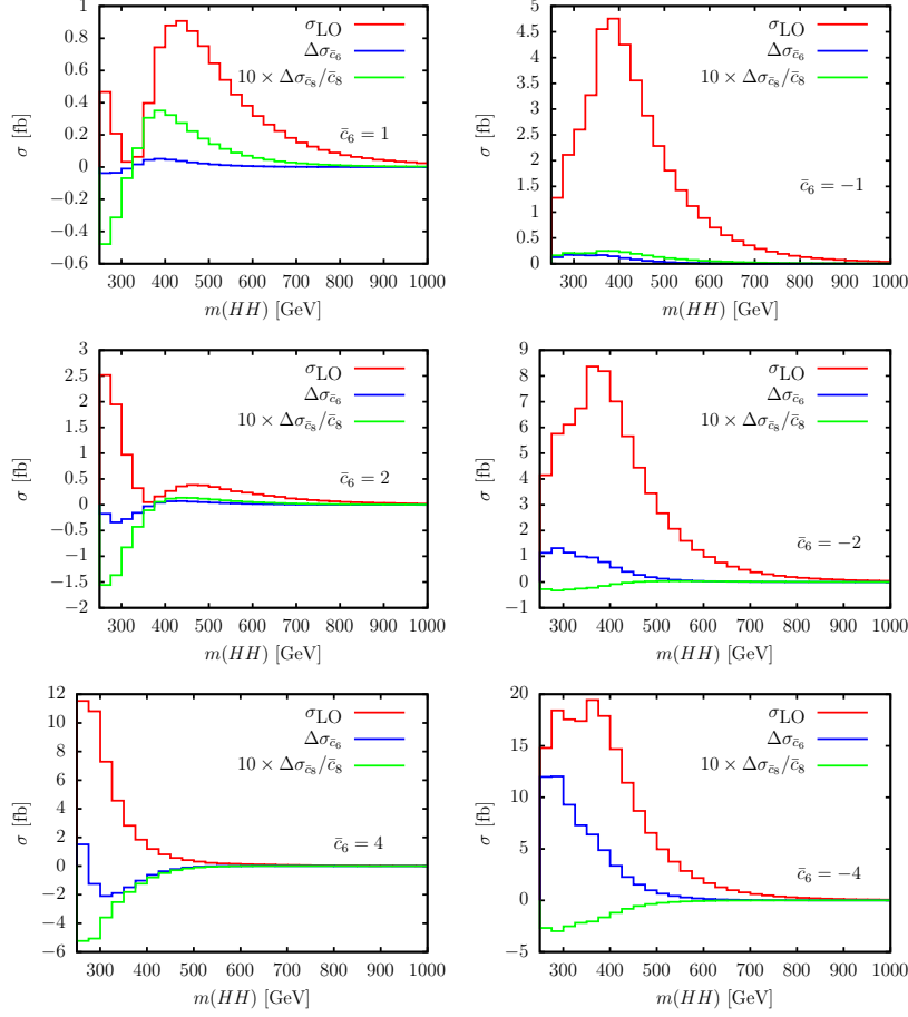
Figure 3.22: The m(HH) distribution of different contributions ( \sigma_{LO} , \Delta\sigma_{\bar{c}_6} , \Delta\sigma_{\bar{c}_8}/\bar{c}_8 ) at 14 TeV hadron collider for different \bar{c}_6 values.
