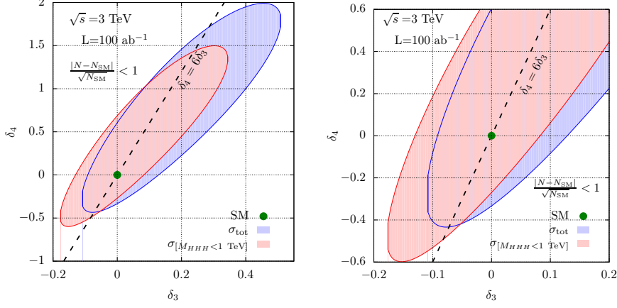
Figure 5.13: Left: 1\text{-}\sigma exclusion plot for the anomalous Higgs self-couplings in terms of the standard deviations |N - N_{\text{SM}}|/\sqrt{N_{\text{SM}}} from the SM (green dot), where the event numbers N refer either to \sigma(\mu^+\mu^- \rightarrow HHH\nu\bar{\nu}) , for M_{\bar{\nu}\nu} \gtrsim 150\text{GeV} (blue area), or to the same cross section with an upper cut of 1 TeV on the HHH invariant mass (red area). Right: same plot zoomed around the SM configuration. The integrated luminosity assumed is about 20 times larger than the reference luminosity in table 5.1.
