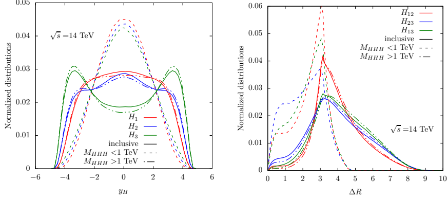
Figure 5.7: Higgs rapidity (left) and Higgs-pair \Delta R (right) distributions in \mu^+\mu^- \rightarrow HHH\nu\bar{\nu} , in the SM, at \sqrt{s} \simeq 14 TeV, for M_{\nu\bar{\nu}} \gtrsim 150 GeV. The index 1 refers to the highest- p_T Higgs, while the index 3 refers to the lowest- p_T Higgs. The solid lines stand for the inclusive distributions, the dashed (dotdashed) lines correspond to applying a further cut M_{HHH} < (>) 1 TeV.
