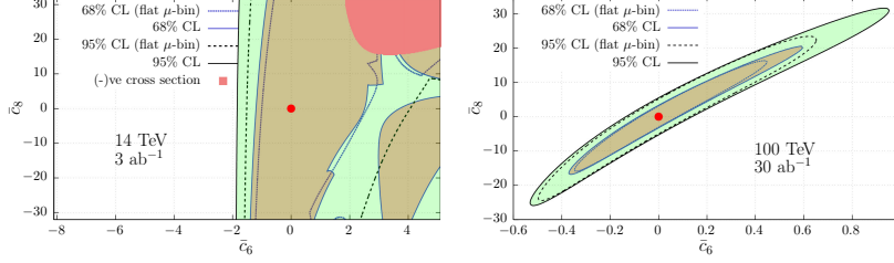
Figure 3.26: Expected 1\sigma and 2\sigma bounds in the (\bar{c}_6, \bar{c}_8) plane at 14 TeV(left) and 100 TeV(right), assuming \bar{c}_6^{\text{true}} = \bar{c}_8^{\text{true}} = 0 .
