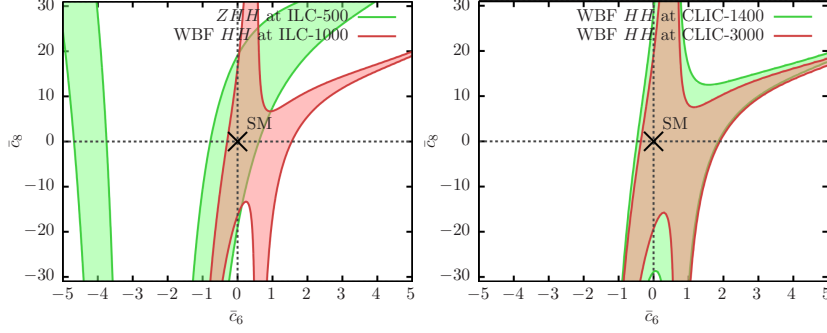
Figure 4.11: 2\sigma bounds in the (\bar{c}_6, \bar{c}_8) plane assuming SM cross sections for double Higgs production in the Scenario 2 described in the text. Left: ZHH at ILC-500 and WBF\ HH at ILC-1000. Right: WBF\ HH at CLIC-1400 and CLIC-3000.
