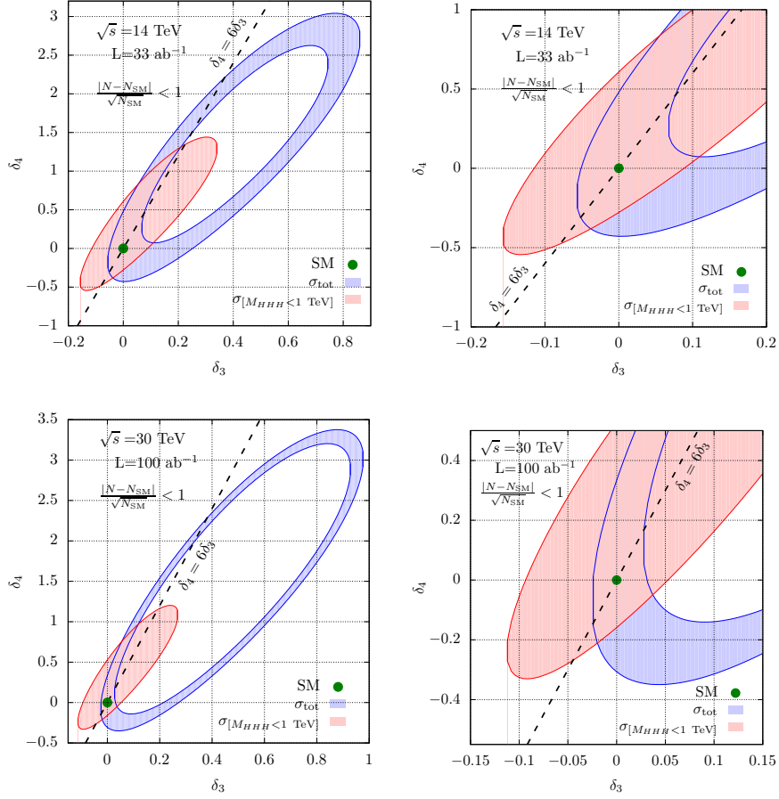
Figure 5.12: Left: 1- \sigma exclusion plots for the anomalous Higgs self-couplings in terms of the standard deviations |N - N_{\text{SM}}|/\sqrt{N_{\text{SM}}} from the SM (green dot), where the event numbers N refer either to \sigma(\mu^+\mu^- \rightarrow HHH\nu\bar{\nu}) , for M_{\bar{\nu}\nu} \gtrsim 150\text{GeV} (blue area), or to the same cross section with an upper cut of 1 TeV on the HHH invariant mass (red area). Right: same plots zoomed around the SM configuration.
