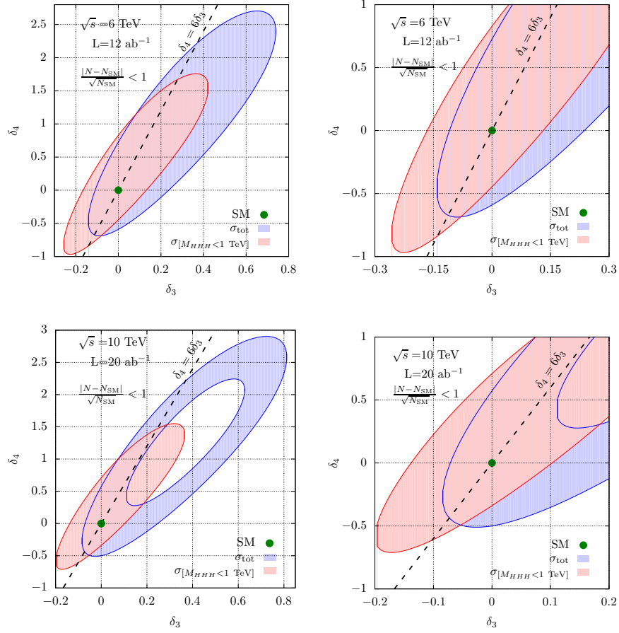
Figure 5.11: Left: 1- \sigma exclusion plots for the anomalous Higgs self-couplings in terms of the standard deviations |N - N_{\text{SM}}|/\sqrt{N_{\text{SM}}} from the SM (green dot), where the event numbers N refer either to \sigma(\mu^+\mu^- \rightarrow HHH\nu\bar{\nu}) , for M_{\nu\bar{\nu}} \gtrsim 150\text{GeV} (blue area), or to the same cross section with an upper cut of 1 TeV on the HHH invariant mass (red area). Right: same plots zoomed around the SM configuration.
