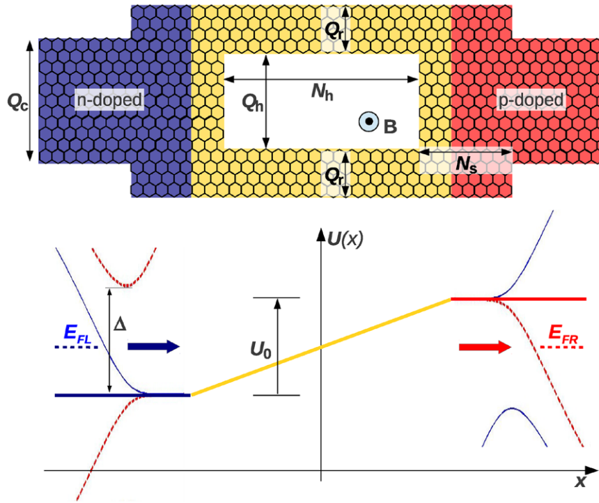
Figure 1. Schematic of the graphene nanoribbon ring considered in this work and its energy band profile. Q_r , Q_c and Q_h characterize the width of the ring, of the contact graphene nanoribbons and of the hole, respectively. N_h defines the length of the hole and N_s stands for the size of side nanoribbons along the transport direction. U_0 is the potential difference between p-doped and n-doped zones, while E_{FL(R)} denotes the Fermi level in the left (right) contact.
