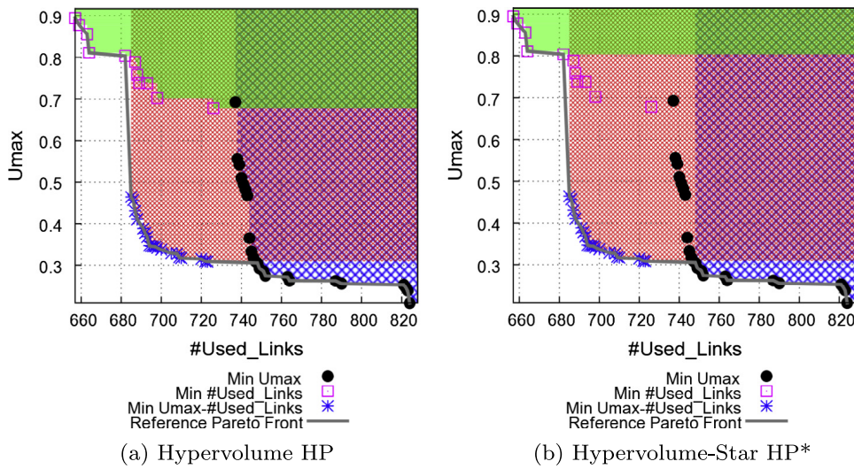
Fig. 4. ( U_{max} , #Links) measurement on cloud data center.
