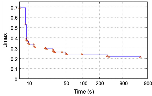
Fig. 1. Improvement of U_{max} over execution time.
