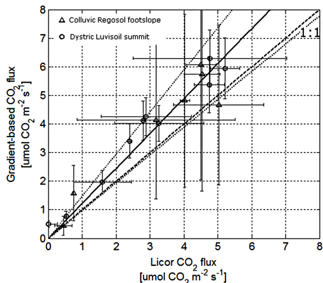
Figure 5. Agreement between soil surface \text{CO}_2 fluxes directly measured with surface survey chambers (horizontal axes) and \text{CO}_2 fluxes calculated according to the gradient-based method (vertical axes) using the Moldrup et al. (2000) diffusivity model. The straight dashed line is the 1 : 1 ideal regression (perfect fit). The straight line is the fitted regression. The dotted straight lines represent a 25 % relative error interval around the fitted regression.
