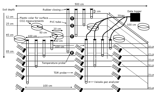
Figure 4. Schematic description of the experimental plot (sampling design) at each slope position showing how temperature, VWC, CO 2 concentrations and CO 2 fluxes probes collocate with each others. Probes have been inserted at different locations both vertically and horizontally. Consequently, all of them are not in the same plane (i.e. depth lines with axes labels on the right hand-side illustrate the foreground profile and depth lines with axes labels on the left hand-side illustrate the background profile).
