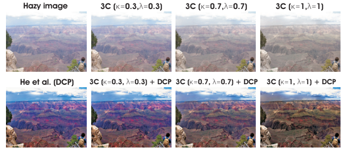
Fig. 7. The impact of \kappa and \lambda parameters. In Equation 2 the parameters \kappa and \lambda define the level of compensation. The compensation increases proportionally to the value of the \kappa and \lambda parameters. Setting \kappa=\lambda=0.7 generally results in the most pleasant images.
