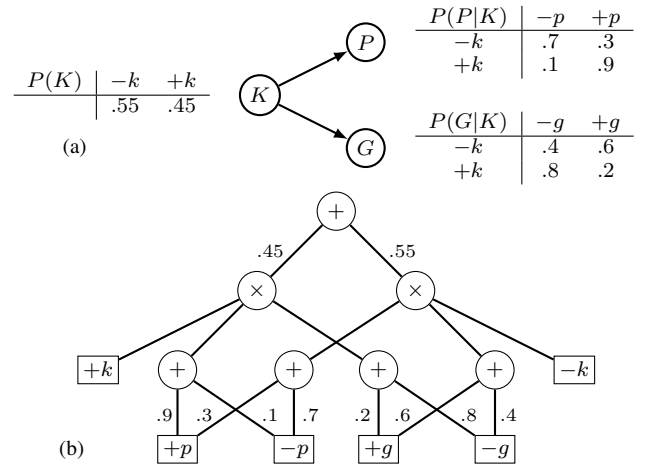
Fig. 2: (a) A Bayesian network encoding a distribution with three variables and (b) An equivalent probabilistic circuit.
