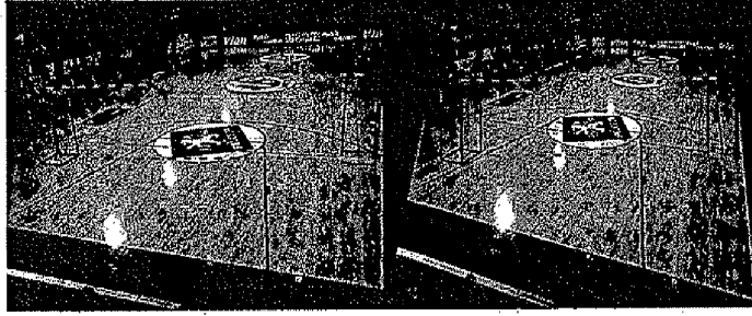
Fig. 3. Efficient computation of the ground occupancy mask: the original view (on the left) is mapped to a plane through a combination of homographies that are chosen so that (1) verticality is preserved during projection from 3D scene to transformed view, and (2) ratio of heights between 3D scene and projected view is preserved for objects that lies on the same line in the transformed view.
