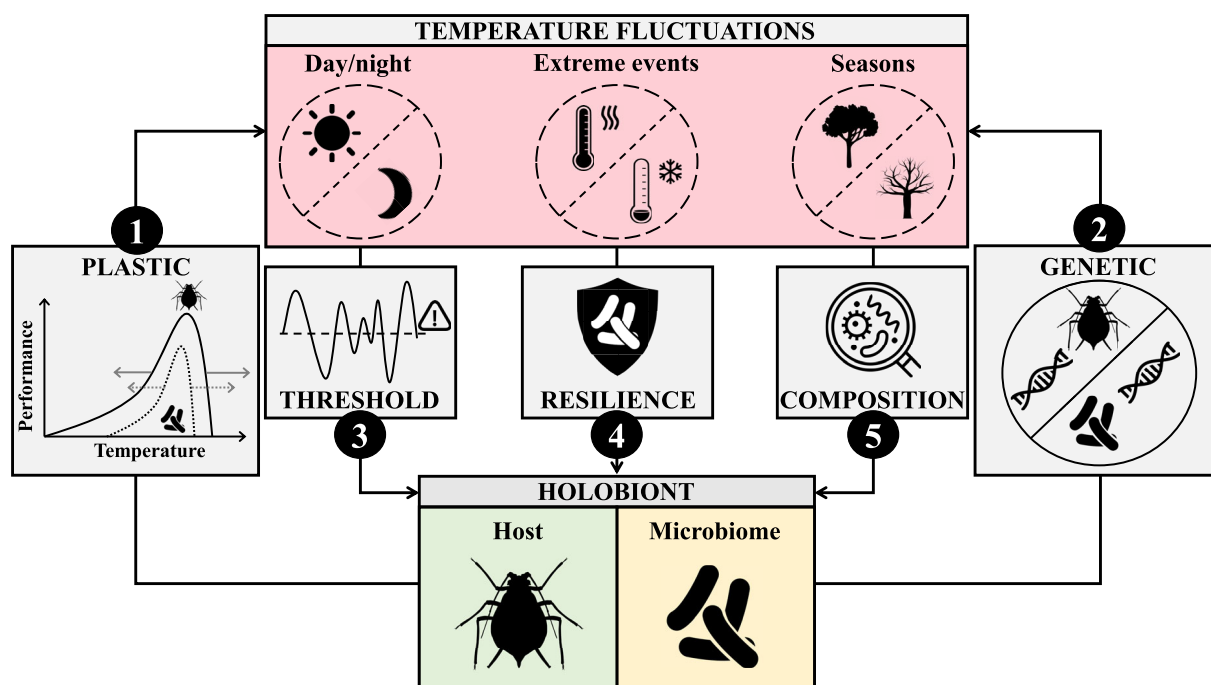
Fig. 1. Responses of insect–microbe holobionts to different patterns of temperature fluctuations, and impacts of thermal variability on the outcomes of these partnerships. (1) Plastic responses can operate over short timescales (e.g. within a generation) to enable rapid mitigation of thermal stress through behavioural (thermoregulation) and physiological (acclimation) processes. They are usually described through the lens of thermal performance curves (the relationship between a fitness metric and temperature), which can differ between insect and microbial players. The ecological and molecular mechanisms underlying these holobiont plastic responses need to be thoroughly elucidated, as well as their adaptive significance (fitness consequences) for partners. (2) Genetic (evolutionary) responses consist of long-term modifications of the host and/or the microbiome genomes in response to selective forces driven by temperature fluctuations. The relative contribution of each interacting species to the holobiont genetic adaptation to fluctuating temperatures remains to be examined, with careful considerations of the genetic diversity apparent at the microbiome level (species, strains, patterns of gene expression). (3) Daily thermal range can impact the holobiont through threshold effects, whereby daytime and/or night-time temperatures are stress-inducing when crossing a set of minimal and/or maximal values. The holobiont ability to express protective mechanisms against altered patterns of daily thermal range, in a manner similar to a single thermal shock, should be evaluated. (4) Extreme thermal events, like heat waves and cold spells, should be profoundly disruptive to insect–microbe associations. Future studies could be conducted to test for the resilience of these systems when facing different patterns of thermal extremes (e.g. heat or cold shock, number, duration and temporal sequence of stressful and recovery periods, timing of application during symbiogenesis). (5) Seasonal fluctuations of temperature can alter the composition of microbiome community. Much less is known about their consequences for host physiology and performance, and their potential indirect impacts on microbial dynamics and host vital functions through induction and termination of insect diapause. [Color figure can be viewed at wileyonlinelibrary.com ]
