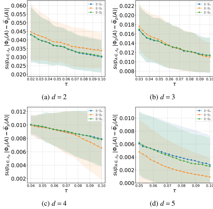
Figure 1: Average errors \sup_{A \in \mathcal{A}} |\hat{\Phi}_p(A) - \Phi_p(A)| with p \in \{1, 2, \infty\} , in dimension d = 2 (top left panel), d = 3 (top right panel), d = 4 (bottom left panel) and d = 5 (bottom right panel), as a function of \tau . Colored intervals represent standard deviations of errors over 500 independent replications.
