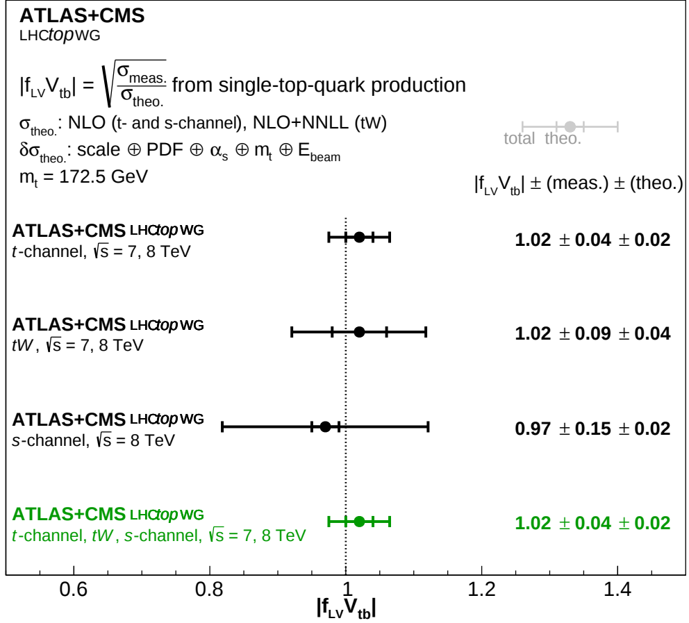
Figure 4: The combined |f_{LV} V_{tb}| value extracted from the t -channel and tW cross-section measurements at \sqrt{s} = 7 and 8 \text{ TeV} from ATLAS and CMS, as well as the ATLAS s -channel measurement at \sqrt{s} = 8 \text{ TeV} , is shown together with the combined |f_{LV} V_{tb}| values for each production mode. The theoretical predictions for t -channel and s -channel production are computed at NLO accuracy, while the theoretical predictions for tW are calculated at NLO+NNLL accuracy. The \sigma_{\text{theo.}} uncertainties used to compute |f_{LV} V_{tb}| include scale, PDF+ \alpha_s , m_t , and E_{\text{beam}} variations.
