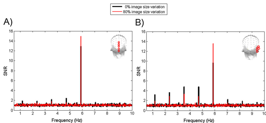
Figure 2 Grand-averaged SNR spectra (displayed between 0.5 and 10 Hz) over medial occipital (A) and right occipito-temporal (B) regions for the conditions 0 and 80% image size variation. 3D maps display electrodes position for each ROI. The EEG spectra demonstrate clear responses at the two embedded frequencies: base ( F = 5.88 Hz) and oddball frequencies ( 1F/5 = 1.18 Hz, 2F/5 = 2.36 Hz, 3F/5 = 3.50 Hz, 4F/5 = 4.70 Hz, 6F/5 = 7.05 Hz, etc.). SNR = 1 at noise level.
