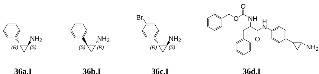
Figure 21.I. Chemical structures of tranlylcypromine derivatives ( 36a-d.I ).
