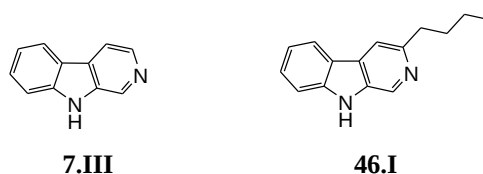
Figure 20.III. Chemical structures of norharman ( 7.III ) and 3-butyl- \beta -carboline ( 46.I ).
