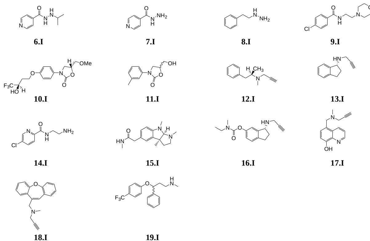
Figure 5.I. Chemical structures of iproniazid ( 6.I ), isoniazid ( 7.I ), phenelzine ( 8.I ), moclobemide ( 9.I ), befloxatone ( 10.I ), toloxatone ( 11.I ), l -deprenyl ( 12.I ), rasagiline ( 13.I ), lazabemide ( 14.I ), physostigmine ( 15.I ), ladostigil ( 16.I ), M30 ( 17.I ), CGP 3466 ( 18.I ) and fluoxetine ( 19.I ).
