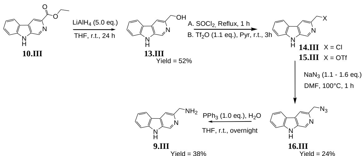
Scheme 7.III. Synthetic pathway to 3-methylamino-β-carboline ( 9.III ).
