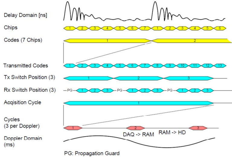
Figure 2.2: Timing concept[2]
