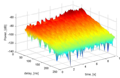
(f) Simulated time-variant PDP, node Rx7
