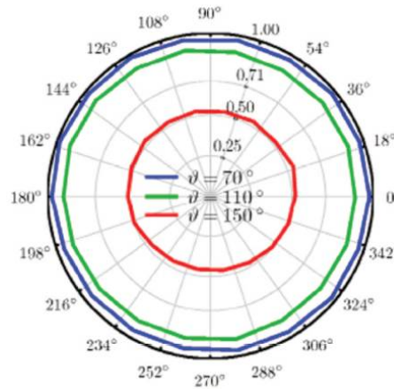
(e) Radiation pattern of the node antenna at 3.8 GHz. Polarization in \vartheta -direction versus \varphi (left) and Polarization in \vartheta -direction versus \vartheta (right)
