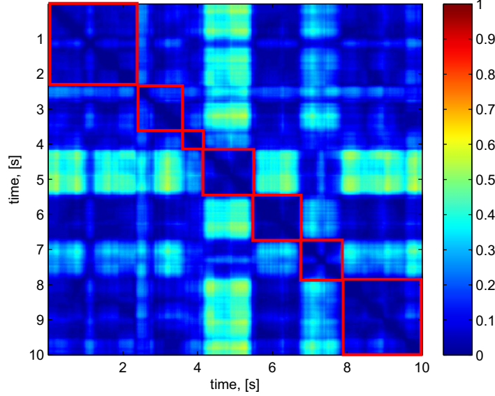
Figure 4.8: Correlation Matrix Distance for 10 seconds of measured channel Tx-Rx6, squared definition of stationarity periods
