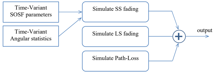
Figure 4.23: Flow-diagram of the channel model
