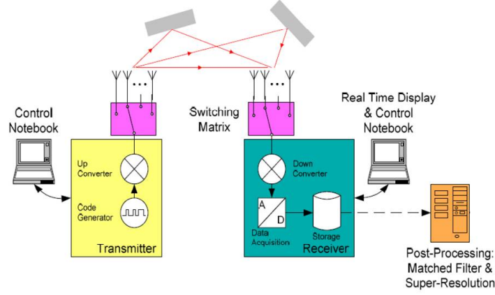
Figure 2.1: Block diagram of the Elektrobitt channel sounder [2]
