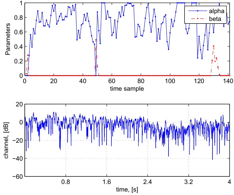
Figure 3.9: Simulated small-scale fading distribution parameters over time for the double-mobile scenario (top). Simulated time-variant components of the channel (small-scale fading and dynamic LS fading) (bottom)
