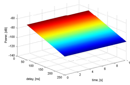
(b) Deterministic PDP, node Rx7
