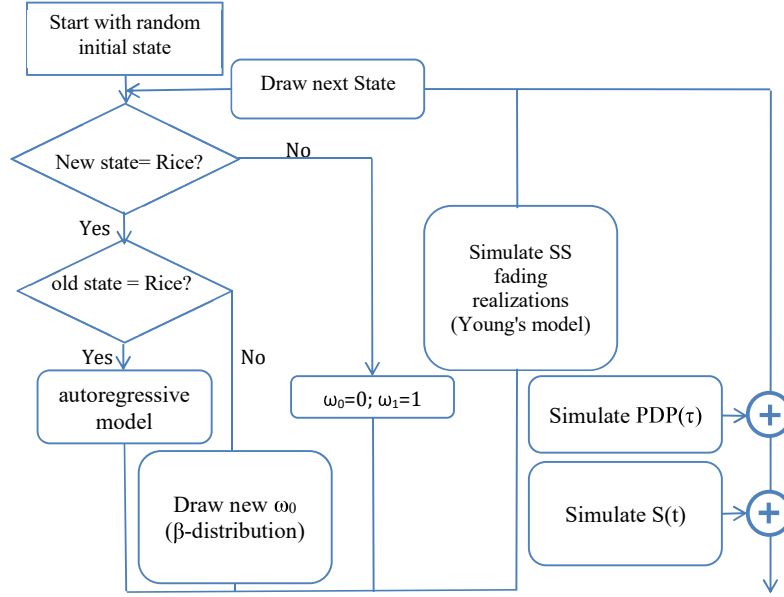
Figure 5.6: Flow diagram of the complete model (Steps A+B)
