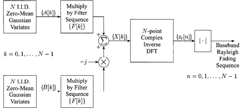
Figure 1.11: Young's model [78]
