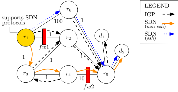
Fig. 1. Example of hybrid SDN network.
