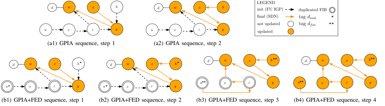
Fig. 5. Application of our procedure to the example in Fig. 2. Fig. 5(a1) and 5(a2) reports the node update sequence as computed by GPIA (phase 1 of our procedure). Fig. 5(b1), 5(b2), 5(b3) and 5(b4) depicts the final operational sequence computed after the application of FED (phase 2 of our procedure).
