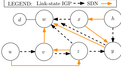
Fig. 2. An example in which no FIB replacement ordering can prevent path inconsistencies. The only applicable approach among prior works is network-wide FIB duplication [17], [2], [5], that comes with high overhead.
