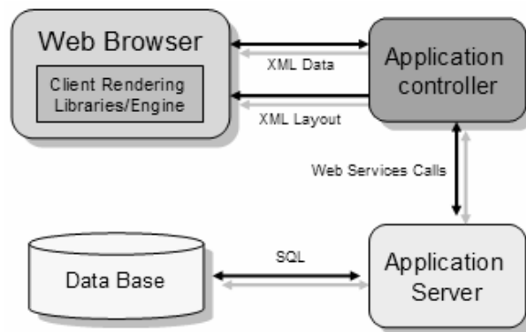
Figure 1: Typical architecture of a RIA application.
