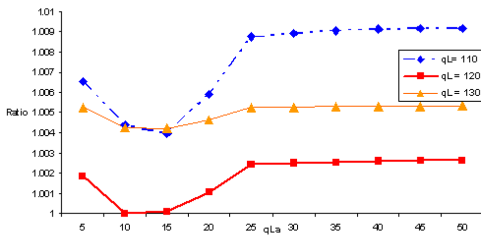
Figure 8: Graph of efficiency ratio for 3 capacities and all additional capacities, p-values < 0.01
