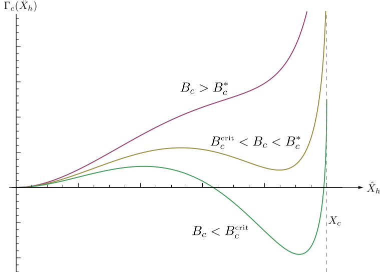
FIG. 2: The Schwarzschild model action \Gamma_c(\hat{X}_h) for 0 \leq \hat{X}_h \leq X_c . Local extrema appear only for B_c below a certain value B_c^* .
