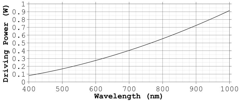
Figure 4.12 – Curve showing the driving power to be applied to the transducer in order to preserve the maximum DE over the tuning range. (TeO 2 AOTF, \alpha = 10^\circ , L_T = 15 mm, H_T = 10 mm)
