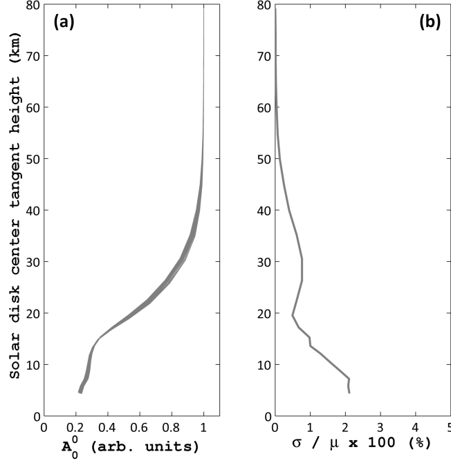
Figure 2.7 – Left panel shows the moment amplitude of the first Zernike polynomial computed for every simulated solar disk image and every profile of the CIRA-86 climatology. At the beginning of the occultation, the weakness of the refraction makes the Zernike moment insensitive to the particular pressure of the upper atmospheric layers. At lower altitudes, the moment starts taking different values for different pressure profiles. This is emphasized in the second panel where the standard deviation of the moment amplitude is compared to the mean value.
