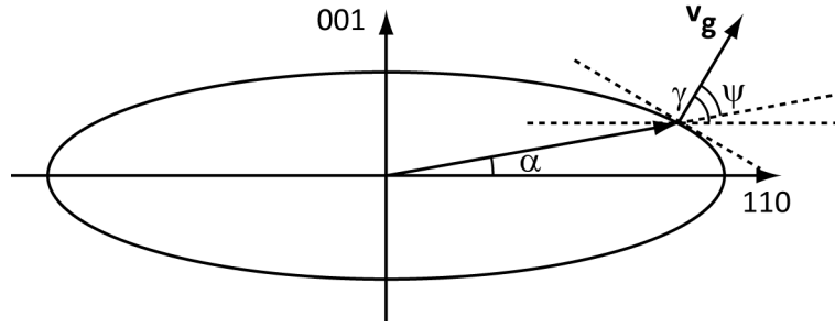
Figure 4.7 – Slowness curve for a \bar{1}10 -polarized shear acoustic wave propagating in the \bar{1}10 plane in \text{TeO}_2 .
