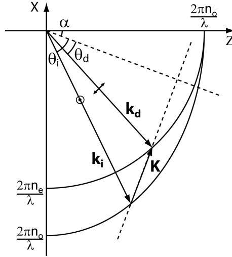
Figure C.1 – Momentum matching diagram in a KDP AOTF.
