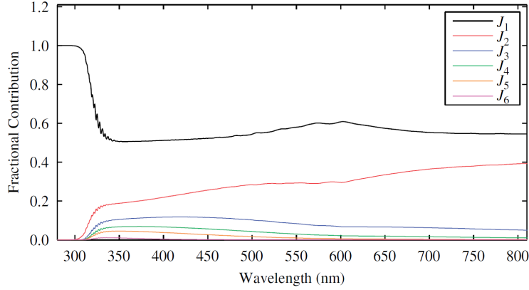
Figure 1.9 – Relative contribution of the scattering orders for a typical measurement geometry of OSIRIS and a tangent point at 25 km. (Reproduced from [11])
