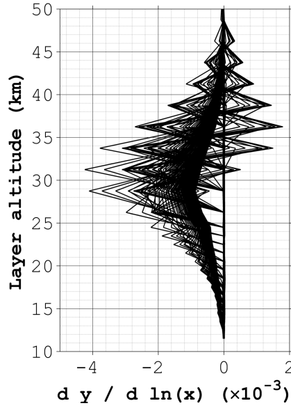
Figure 3.15 – Weighting functions representing the response of the measurement vector to a 5% perturbation of the NO 2 profile.
