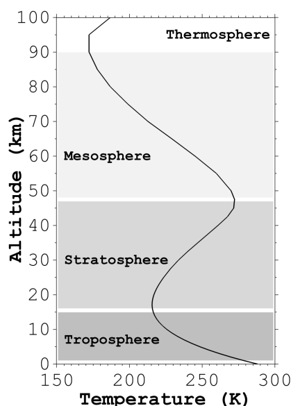
Figure 1.1 – Northern mid-latitude summer atmospheric temperature profile.
