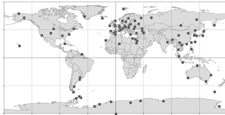
Figure 1.3 – Location of the GAW ground stations having delivered ozone data in 2013.
