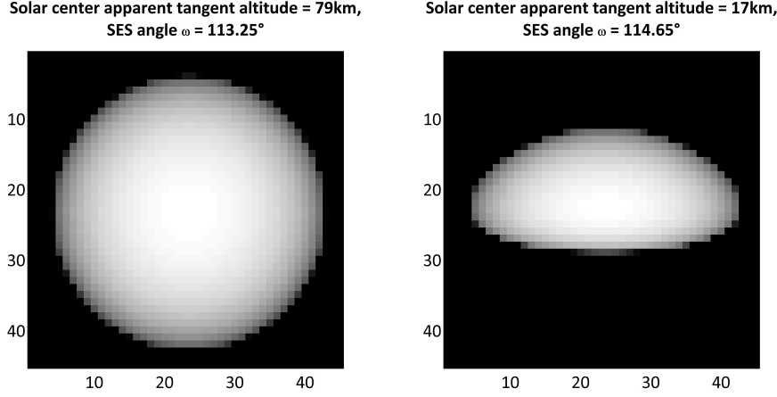
Figure 2.2 – Simulated pictures of the Sun. Left picture shows a high Sun, right picture shows a low Sun already experiencing strong flattening. Notice the asymmetrical flattening.
