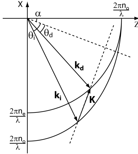
Figure 4.14 – Momentum vector diagram illustrating the birefringent AO interaction in KDP.
