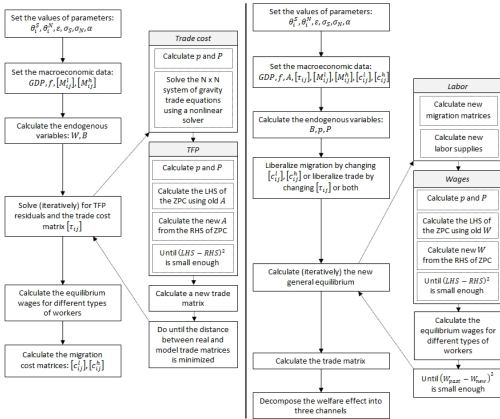
Figure C.1: The calibration (left panel) and the simulation (right panel) algorithms.
