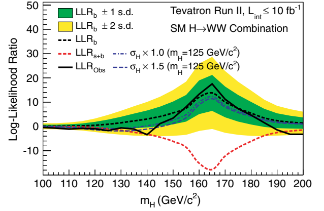
FIG. 11 (color online). LLR as a function of Higgs boson mass from the combination of CDF's and D0's SM Higgs boson searches focusing on the H \rightarrow W^+W^- decay mode. The solid line shows the observed LLR values, the dark short-dashed line shows the median expectation assuming no Higgs boson signal is present, and the dark- and light-shaded bands correspond, respectively, to the regions encompassing 1 and 2 s.d. fluctuations around the background-only expectation. The red long-dashed line shows the median expectation assuming a SM Higgs boson signal is present at each value of m_H in turn. The blue lines show the median expected LLR assuming the SM Higgs boson is present at m_H = 125 \text{ GeV}/c^2 with signal strengths of 1.0 times (short-dashed) and 1.5 times (long-dashed) the SM prediction.
