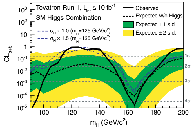
FIG. 8 (color online). The solid black line shows the signal-plus-background p -value as a function of m_H for all of CDF's and D0's SM Higgs boson searches in all decay modes combined. The dotted black line shows the median expected values assuming no SM signal is present, evaluated separately at each m_H . The associated dark- and light-shaded bands indicate the 1 and 2 s.d. fluctuations of possible experimental outcomes under this scenario. The blue lines show the median expected p -values assuming the SM Higgs boson is present with m_H = 125 \text{ GeV}/c^2 at signal strengths of 1.0 times (short-dashed) and 1.5 times (long-dashed) the SM prediction.
