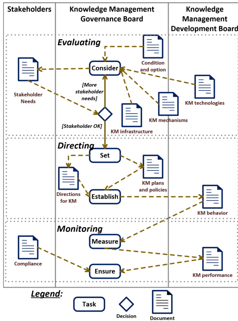
Figure 5: GI-Tropos Knowledge Management Governance Workflow
