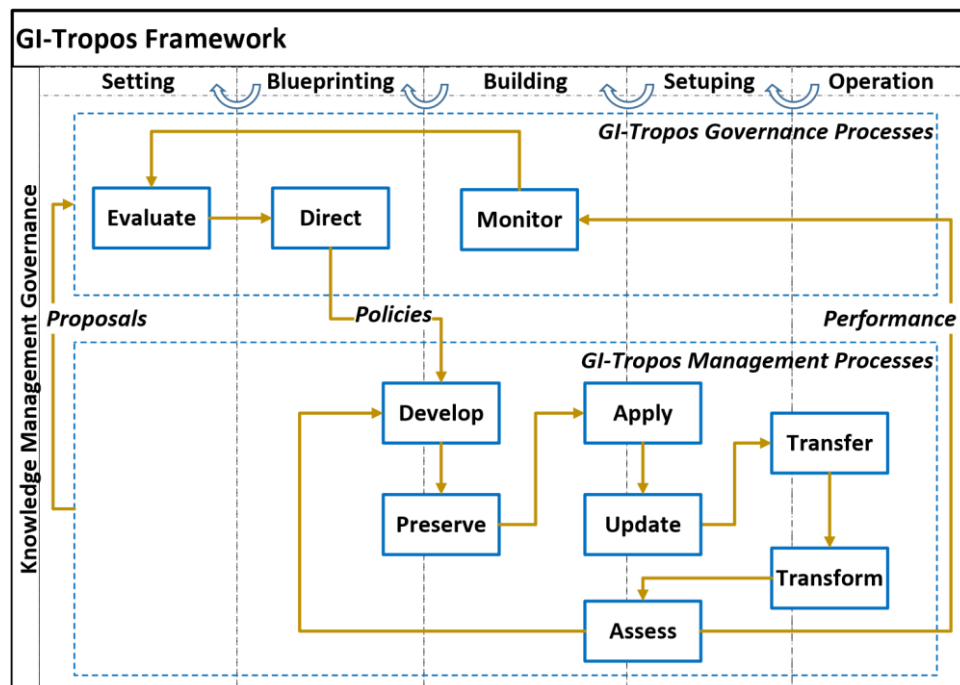
Figure 2: GI-Tropos Knowledge Management Governance Alignment Model
