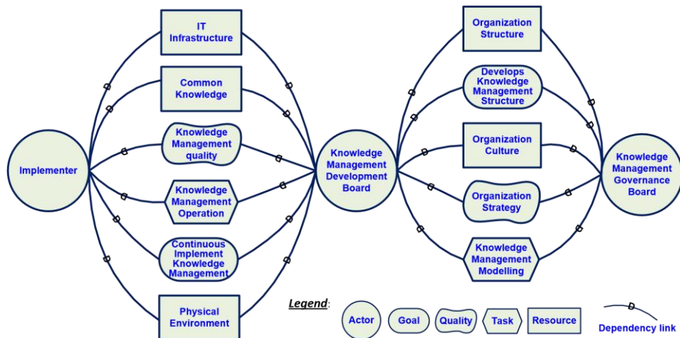
Figure 3: GI-Tropos Knowledge Management Governance Strategic Dependency Model
