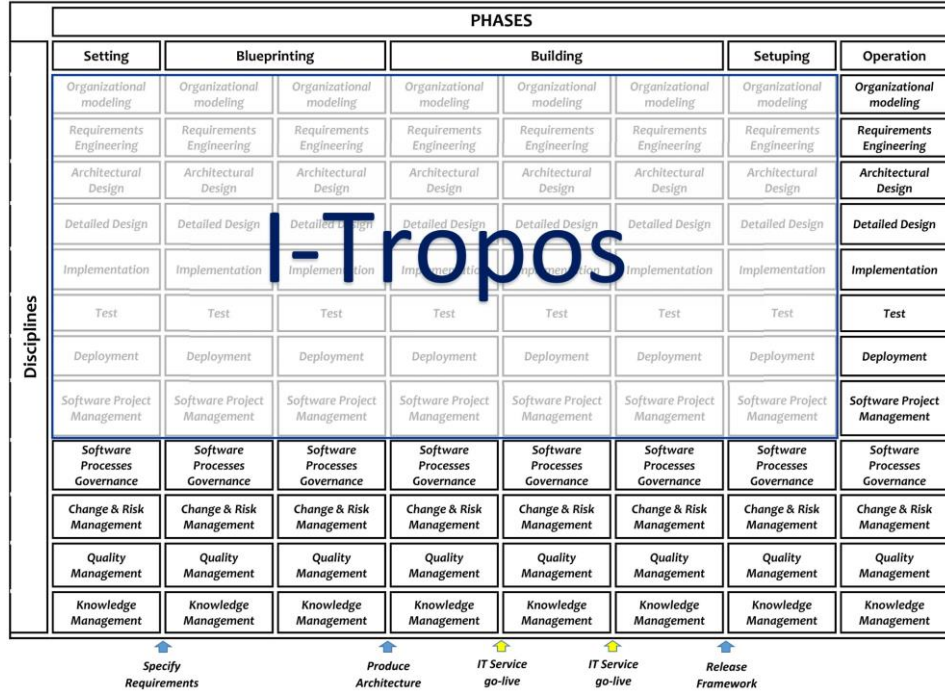
Figure 2: GI-Tropos iterative process framework
