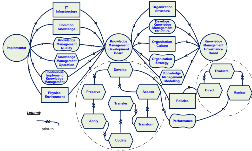
Figure 4: GI-Tropos Knowledge Management Governance Strategic Rationale Model
