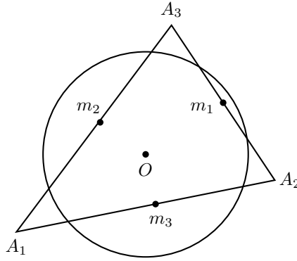
FIGURE 2. The triangle \triangle containing the line segments, and the ball B .
